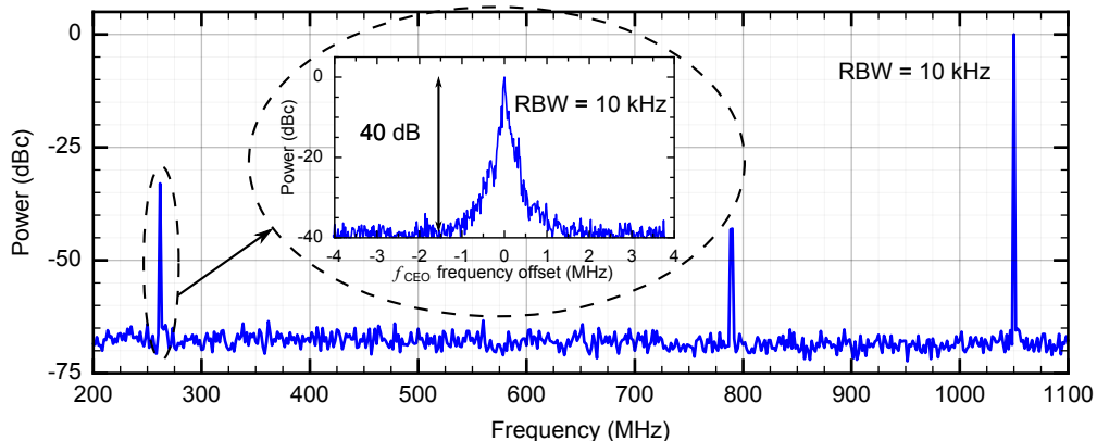
Fig. 4. RF spectrum of the signal at the output of the f -to- 2f interferometer showing a CEO frequency of \sim 266 MHz. The inset displays a zoom on the CEO beat showing an SNR of 40 dB in a RBW of 10 kHz.
