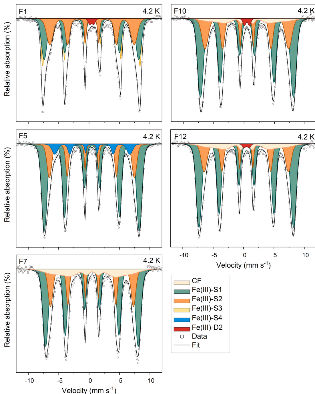
Fig. 6. Mössbauer spectra and fits of selected floc samples collected at 4.2 K. Fit parameters are presented in Table 3. Species assignments: Fe(III)-S1 = ferrihydrite, Fe(III)-S2 = lepidocrocite, Fe(III)-S3 = goethite, Fe(III)-S4 = Fe in clays, Fe(III)-D2 = Fe(III) associated to organic matter, CF = collapsed feature. Fit parameters are detailed in Table 3.
