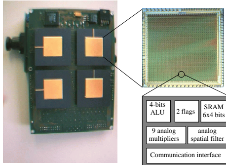
Fig. 1. ProtoEye platform.
