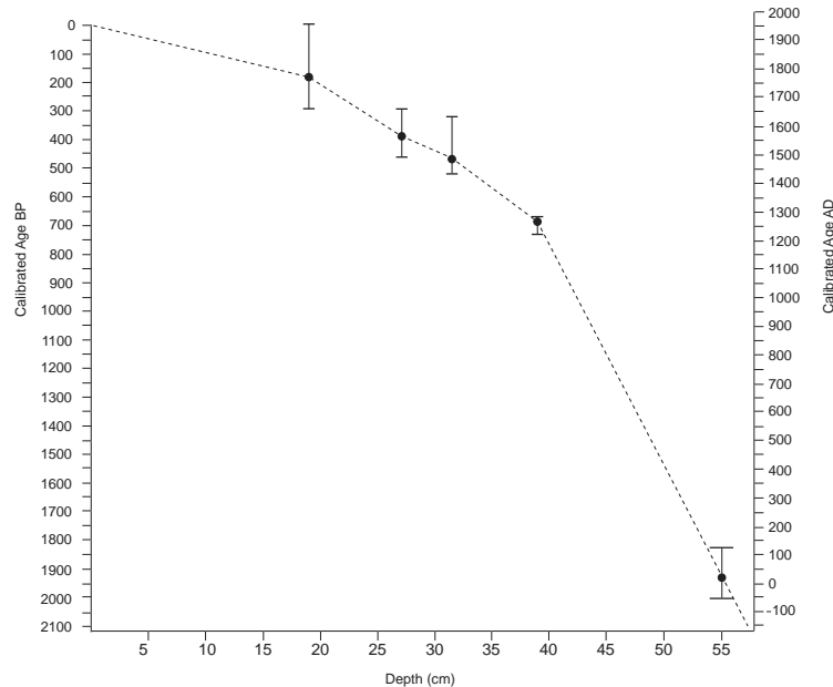
Fig.4. 2: Depth-age relationship for Sourzay peat core. Errors bars show 2\sigma confidence interval. Linear interpolation and extrapolation used to infer the age of pollen samples is shown with line.
