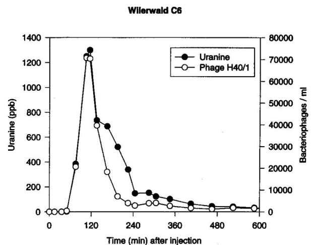
Fig. 6 Uranine and bacteriophage breakthrough curves in the C gallery well C6 at the Wilerwald site (about 12m from the injection point).
