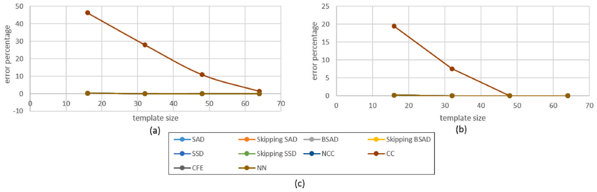
Fig. 12. (a) Results for test case 7 with the original TI, (b) Results for test case 8 with the normalized TI.
