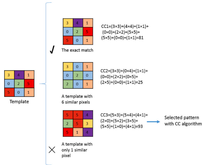
Fig. 15. Calculation of CC for finding the best match for the template. Although the first template is the best match, the CC algorithm selects the worst template as the best match.
