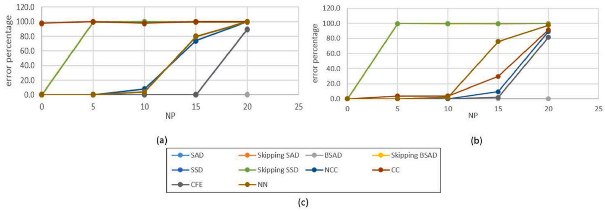
Fig. 14. (a) Results for test case 11, (b) Results for test case 12.
