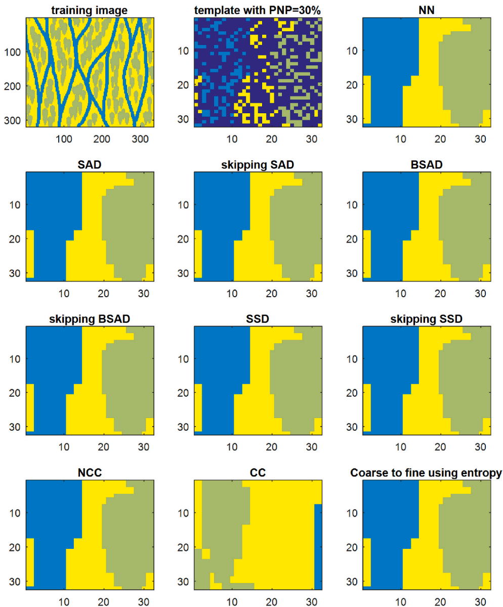
Fig. 16. An Example of results for training image A, template of size 32 \times 32 with PNP = 30 %, and NP = 0 %.
