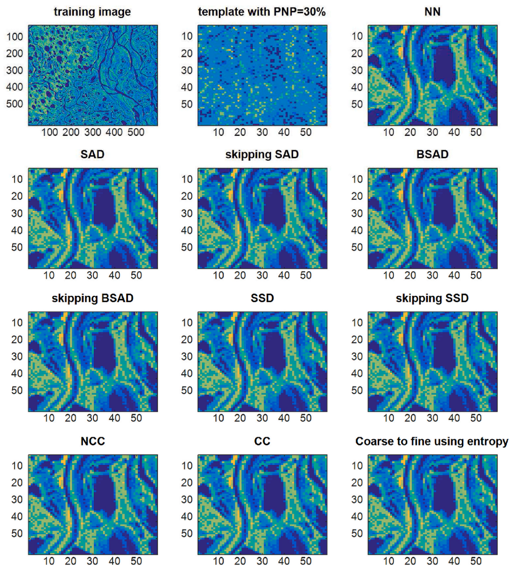
Fig. 19. An Example of results for training image C, template of size 59 \times 59 , with PNP = 30 %, and NP = 0 %.
