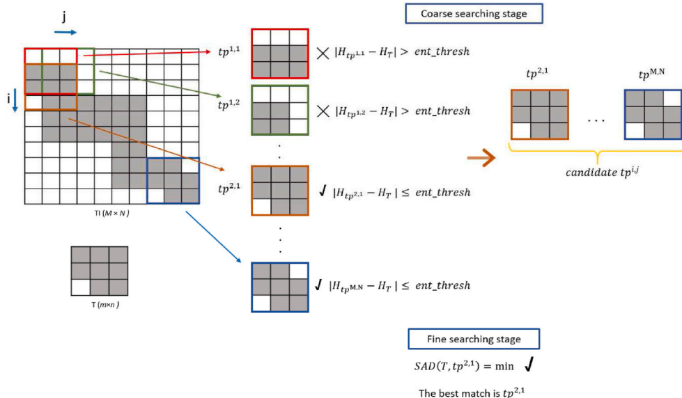
Fig. 3. The procedure of the CFE algorithm.
