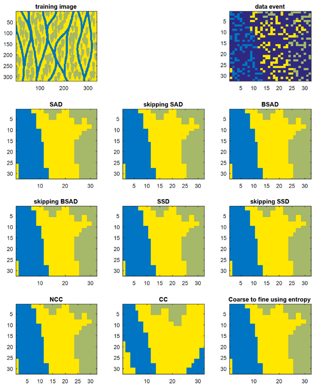
Fig. 17. An Example of results for training image A, template of size 32 \times 32 , with PNP = 30 %, and NP = 10 %.
