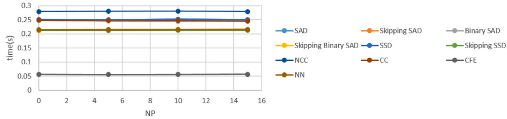
Fig. 10. Efficiency of the ten methods for test case 4.
