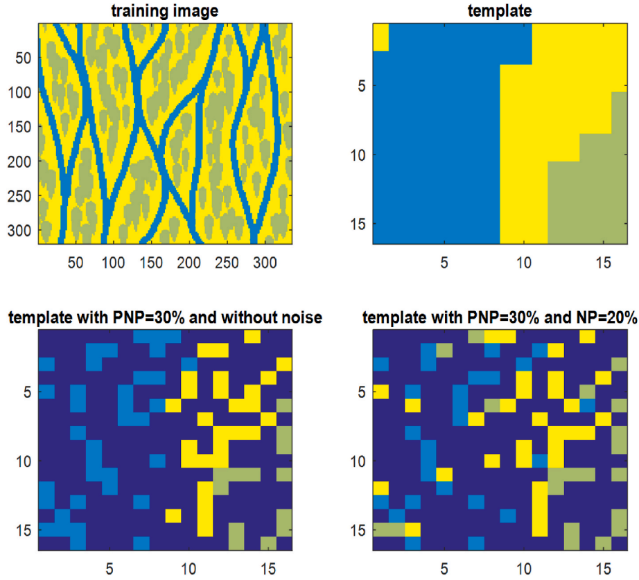
Fig. 6. A 320 \times 335 categorical TI with 3 categories, a 16 \times 16 template from the TI, the template with PNP = 30 % and without noise, and finally, a template with PNP = 30 % and NP = 20 %, (purple regions are unknown).
