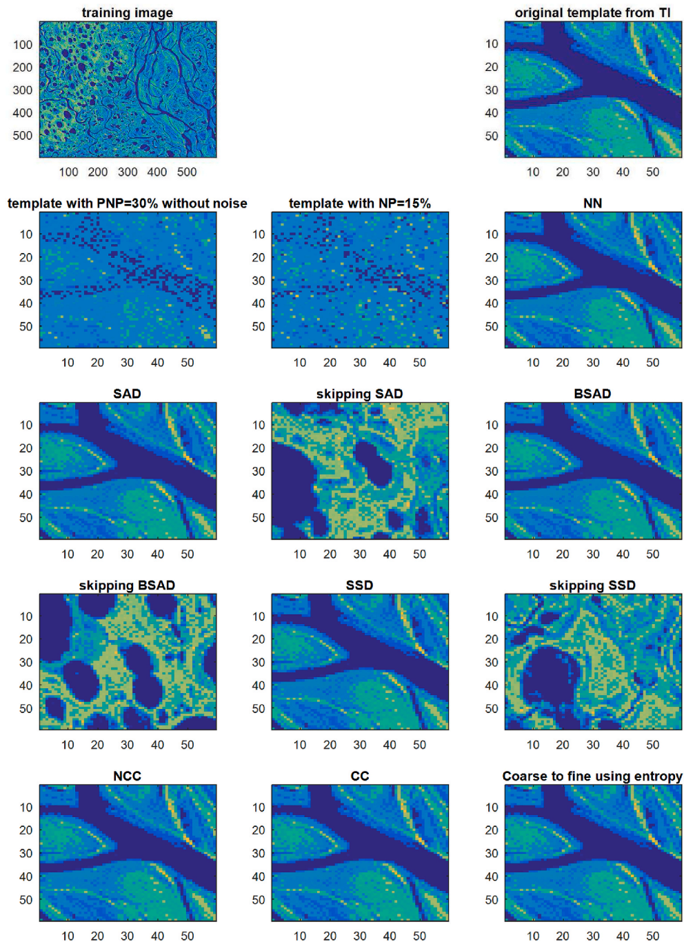
Fig. 21. An Example of results for training image C, template of size 59 \times 59 , with PNP = 30 %, and NP = 15 %.
