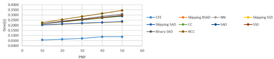
Fig. 9. The efficiency of the ten methods for test case 3.
