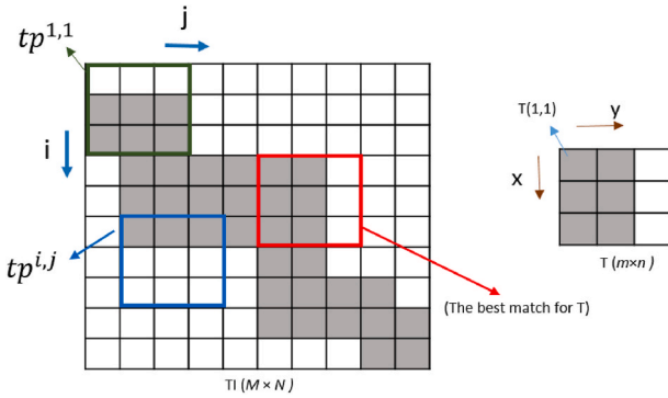
Fig. 2. m \times n template ( T ), M \times N Training Image and tp^{i,j} (a pattern at location (i,j) of Training Image).
