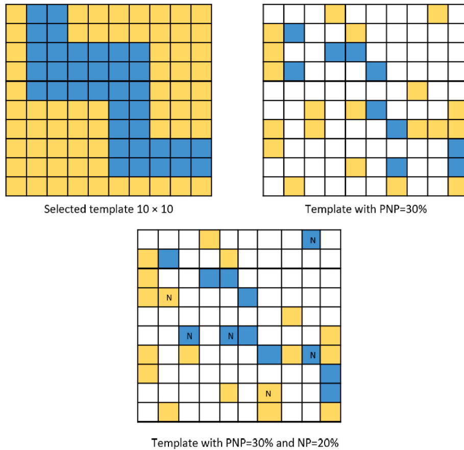
Fig. 5. Example of a selected template, template with PNP = 30 % and the same template with N = 20 % in addition.
