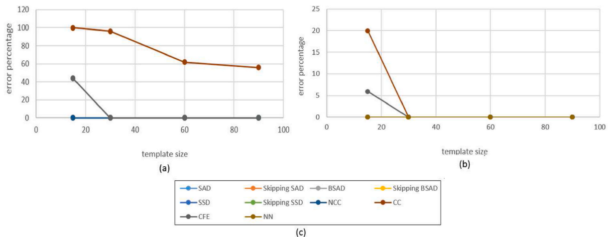
Fig. 11. (a) Results for test case 5 with the original TI, (b) Results for test case 6 with the normalized TI but normalized.
