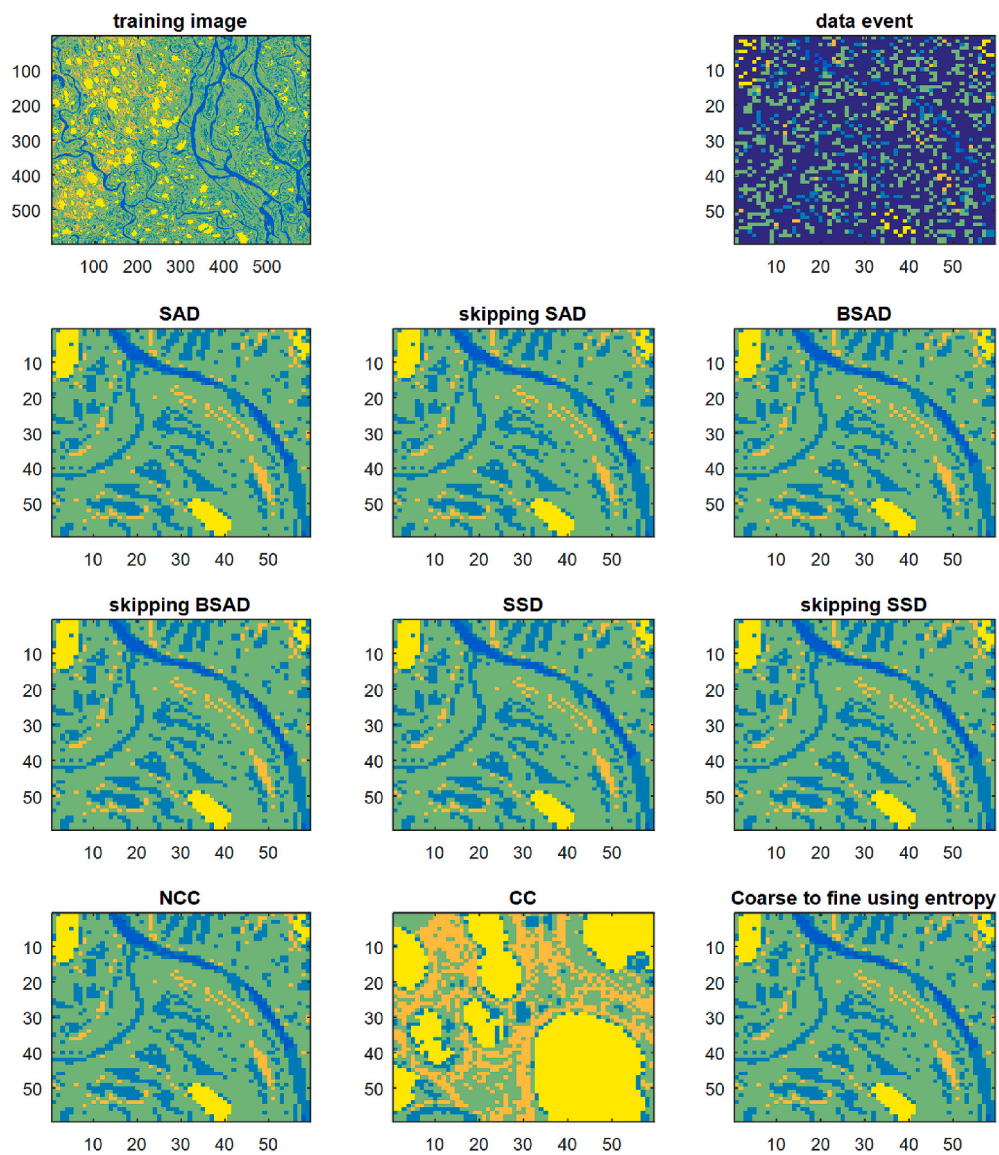
Fig. 18. An Example of results for training image B, template of size 59 \times 59 , with PNP = 30 %, and NP = 5 %.
