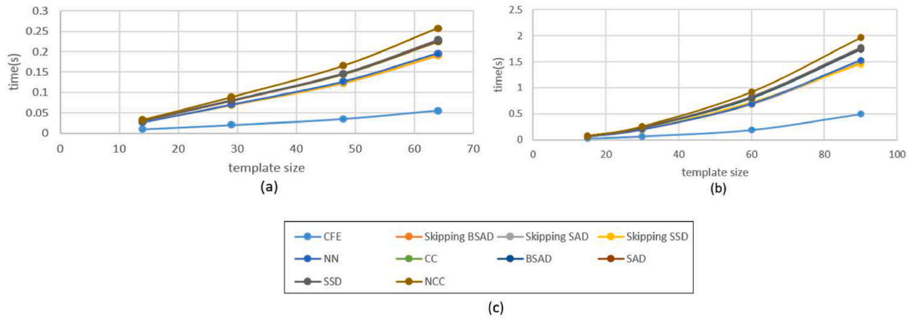
Fig. 8. Comparing the efficiency of TM methods. (a) Results of test case 1 with PNP = 30 and NP = 0, (b) Results for test case 2 with PNP = 30 and NP = 0, (c) Legend for figures a and b.
