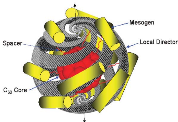
Fig. 4 Proposed helical structure of a supermolecular nanoparticle.
