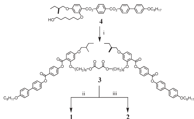
Scheme 1 Reagents and conditions: (i) malonyl chloride, Et 3 N, CH 2 Cl 2 , rt, 63%; (ii) C 60 , I 2 , DBU, toluene, rt, 64%; (iii) C 60 , 9,10-dimethyl-anthracene, toluene, rt, and then 3 , CBr 4 , DBU, rt, 1.4%.
