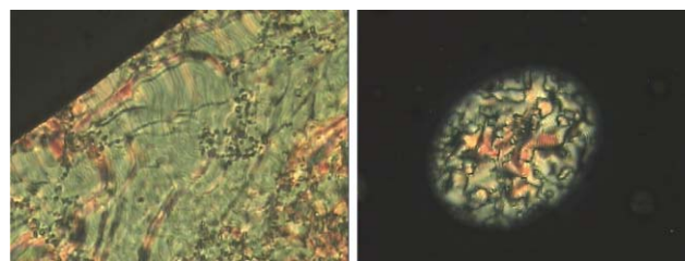
Fig. 2 Textures displayed by 2 : Grandjean-plane texture on the contact area (left) and pseudo-focal conic texture with pitch bands on the non-contact area (right).
