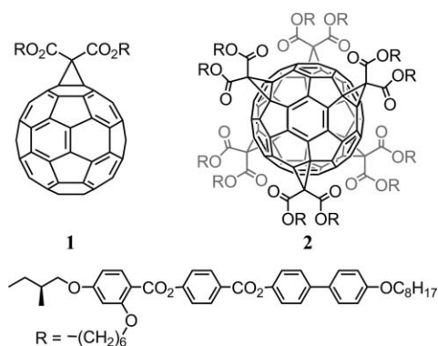
Fig. 1 Structure of mono-adduct 1 and hexa-adduct 2 of fullerene.
