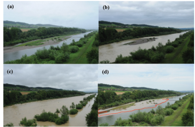
Figure 4. Upstream view of the main island of the Swiss River Thur monitored with high-resolution remotely controllable digital cameras (see Pasquale et al., 2011 for details). The sequence (a–d) shows a compilation of the inundation dynamics during the flood in July 2009 (peak flow of 748 \text{ m}^3 \text{ s}^{-1} ), which resulted in a complete flooding of the restored corridor (c), causing substantial morphologic changes and removal of young vegetation (d). The red contour line in panel (d) shows the comparison with the shoreline of the sediment bar before the flood (a) for the same flow rate.
