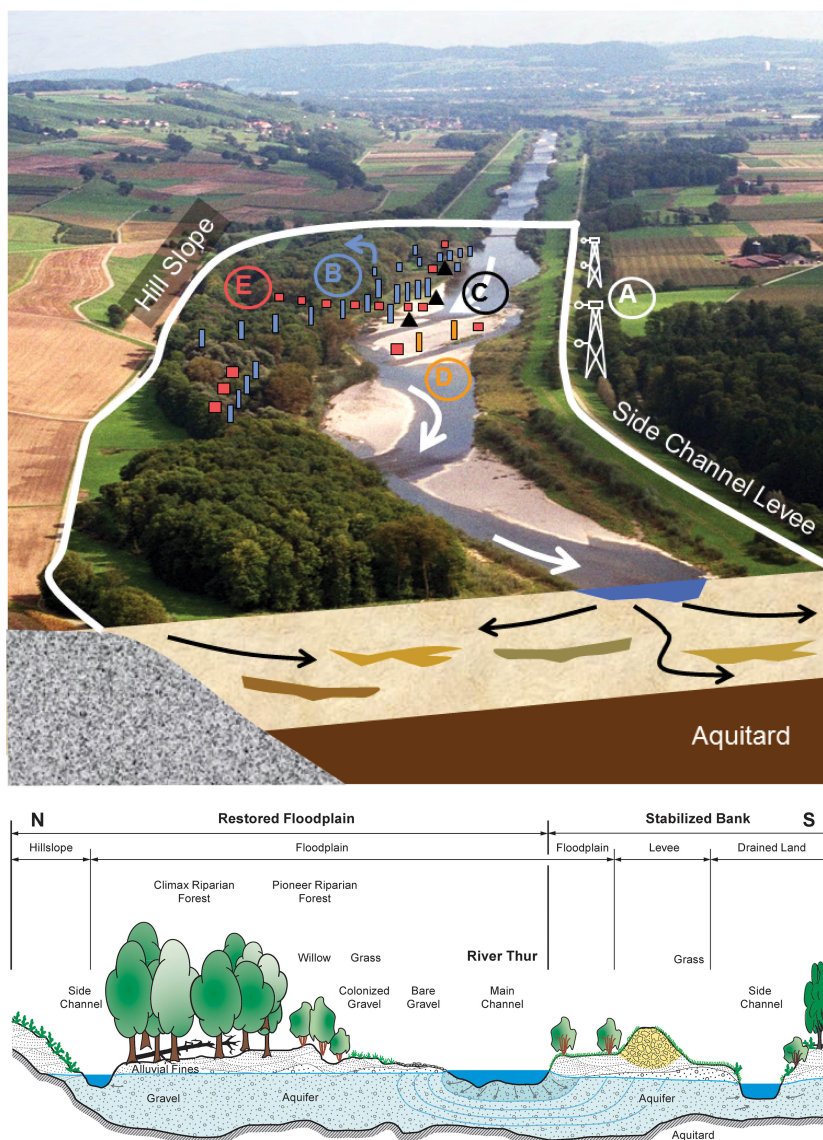
Figure 3. Instrumented field site at the Swiss River Thur close to Niederneunforn ( 47^{\circ}35.4' N , 8^{\circ}46.4' E ) in NE Switzerland with (A) observation towers including cameras, (B) piezometers and wells, (C) geophysical mapping, (D) measurements of meteorological parameters, (E) monitoring of soil parameters (for exact locations see Huber et al., 2012; Shrestha et al., 2014) and (F) biodiversity surveys (for exact locations see Fournier et al., 2012b). The picture was taken by BHAtteam, Frauenfeld. The scheme below visualizes the specific parts of the RECORD field site. It shows a geological cross section representing restored (left) and stabilized/channelized (right) transects at the test site. The restored parts comprise gravel bars developed naturally after restoration, including (i) the gravel zone, sparsely colonized with pioneer plants, (ii) the grass zone, characterized by thick layers of young alluvial overbank sediments and densely colonized with mainly reed canary grass ( Phalaris arundinacea ), (iii) the willow zone, where alluvial sediments were stabilized during restoration by planting young Salix viminalis , and (iv) the alluvial forest dominated by ash and maple and growing on older alluvial sediments.
