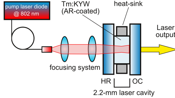
Fig. 1. Schematics of the diode-pumped Tm:KYW laser.
