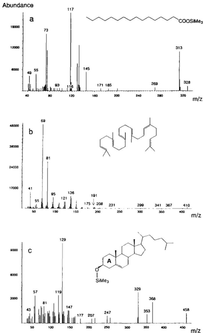
FIG. 3. Mass spectra of the major constituents of the MSTFA-derivatized chloroform samples. (a) Trimethyl silyl derivative of palmitic acid with M^+ 328, intense key fragment ion m/z 313 ( M^+ - 15 ) and base peak m/z 117 of (CO_2SiMe_3)^+ ; (b) squalene with a weak M^+ 410 and key fragment base peak m/z 69 of (C_3H_9)^+ ; and (c) the trimethyl silyl derivative of cholesterol with M^+ 458, the key fragment m/z 368 ( M^+ - 90 ) due to loss of (OSiMe_3)^+ , m/z 329 ( M^+ - 129 ) and base peak m/z 129 of (C_3H_4OSiMe_3)^+ after cleavage of the A ring.
