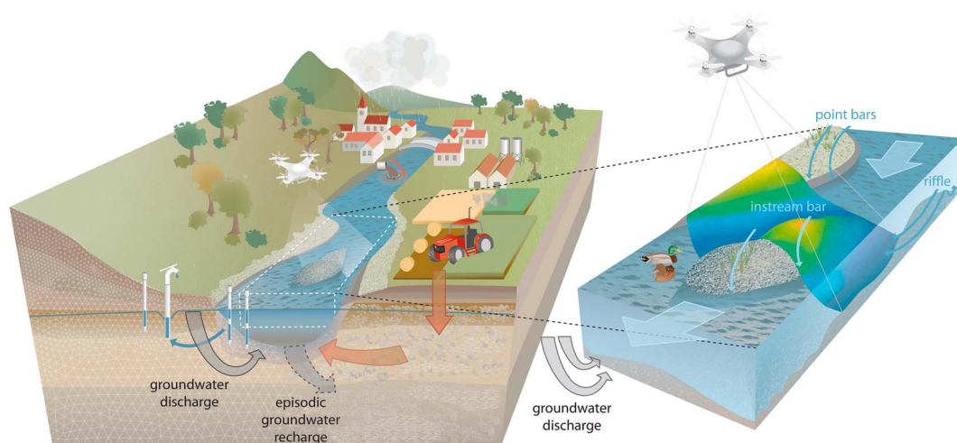
Figure 1. Schematic representation of an anthropogenically modified catchment. The interaction between groundwater and surface water creates numerous challenges related to water quality, quantity, and ecology. The figure illustrates the nested spatial scales of river water and groundwater interactions. (left) The reach scale is illustrated. (right) Hyporheic scale is shown. The technological advances and modeling approaches discussed in this paper provide information across a wide range of scales, and are aimed at a better characterization of the surface (e.g., through drones), the subsurface (e.g., hydraulic observations of water table dynamics or hydraulic properties of the streambed and its conceptualization in numerical flow models), and at measuring exchange fluxes between the surface and the subsurface.
