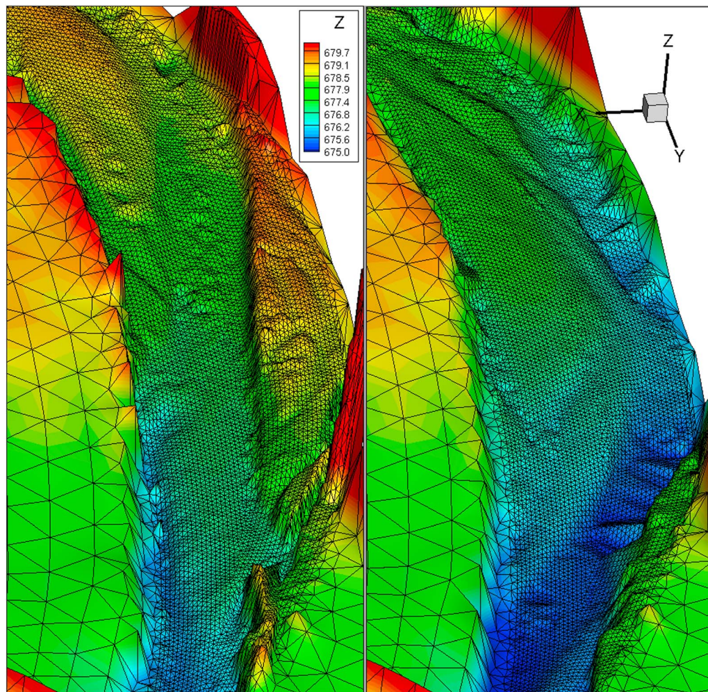
Figure 3. Topography (implemented in a numerical model) of the Emme River (meter above mean sea level), Switzerland, during low flows as an example of a UAV application. The images show a stretch 500 m long and 250 m wide. The two images are based on photogrammetry and show streambed topography (left) before and (right) after a major flood event that modified the streambed. The timing of the image acquisition was critical, as photogrammetry only works for dry streambeds and the Emme River only dries up a few days a year. UAVs provided the flexibility to acquire the data within 24 h after the river dried up. Organizing a helicopter or a plane on such short notice is often impossible.
