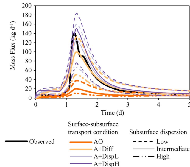
Figure T3.5. Text of the caption directly from the original publication of Liggett et al. [2015]. Influence of subsurface dispersion on the mass flux of total DOC at the catchment outlet.
