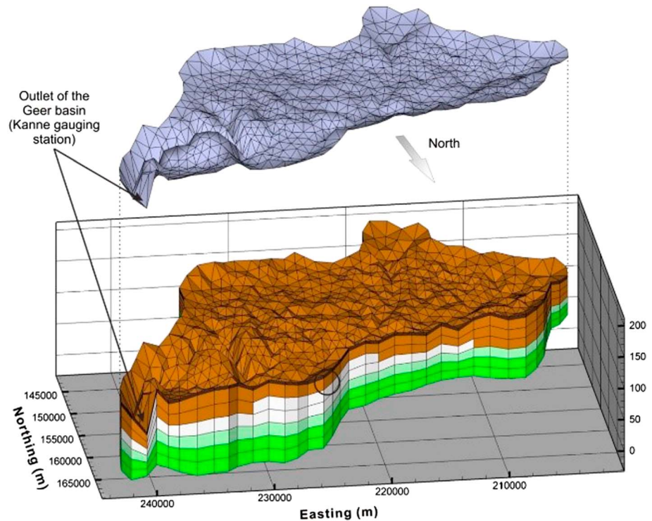
Figure T1.2. Illustration of a discretized river-groundwater model for the 480 km 2 Geer Basin, Belgium (Figure taken from Goderniaux et al. [2009] ). The surface flow domain is discretized in 2-D with triangular elements, and the subsurface flow domain is discretized in 3-D with triangular prisms (6-node elements). The 2-D domain is shown separately here, but it corresponds exactly to the top of the 3-D subsurface mesh.
