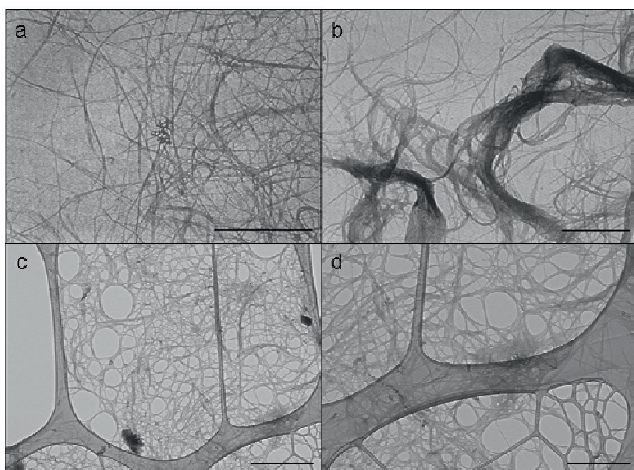
Figure 4 TEM images of SWNT derivative 2a (a), the non functionalized SWNT separated as by product (b) both of them obtained employing Cu grids and SWNT derivative 5a (c and d) obtained employing lacey carbon grids. Scale bars: (a) and (b) 500 nm, (c) and (d) 1000 nm.
