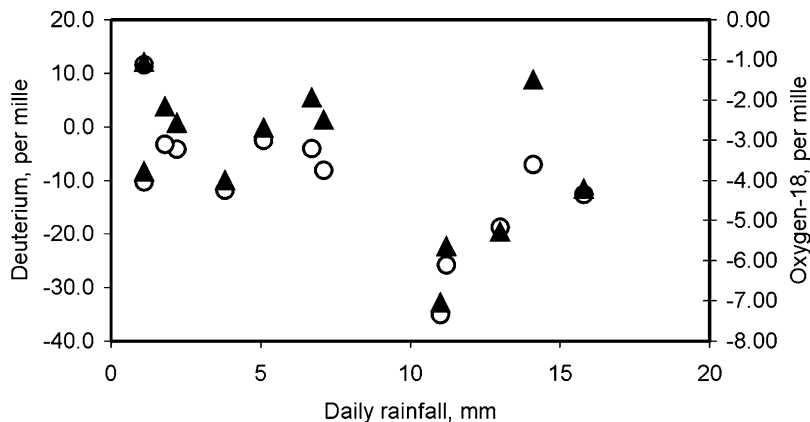
Fig. 5. Isotopic compositions ( \delta D —circles, \delta^{18}O —triangles) of single rainfalls versus daily rainfall amounts (mm) at the Saittos meteorological station (640 m a.s.l.) in October–November 2001.
