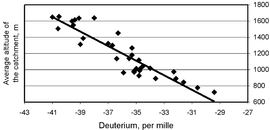
Fig. 8. Regression line between \delta D in 33 springs and average altitudes of their catchments.
