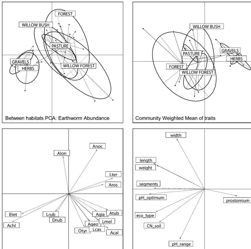
Fig. 3. Principal component analyses (PCA) of earthworm abundance and community weighted means of traits data from the Thur River site. Ellipses highlight the different habitats; and arrows show the position of species or traits within the ordination space. Species name abbreviations are composed of the first letter of the genera and the three first letters of the species name.
