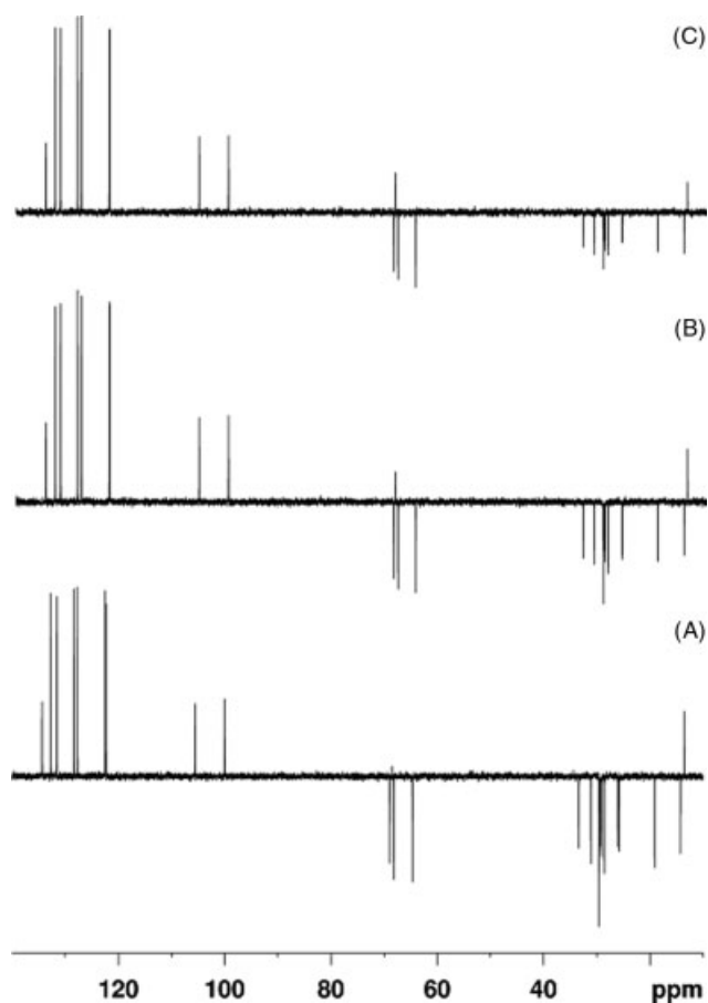
Figure 6. DEPT135 and ACCORDEPT135 spectra of molecule 1 dissolved in CD 2 Cl 2 . (A) DEPT135 optimized for a ^1J_{CH} coupling constant of 145 Hz. (B) ACCORDEPT135 recorded using the DCT method. (C) ACCORDEPT135 recorded using the DCC method. For both ACCORDEPT, the range of ^1J_{CH} coupling constants sampled is 120–260 Hz. It has been sampled using 32 values equally spaced in time or frequency. Other experimental parameters are given in the experimental part.
