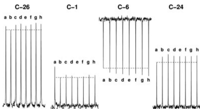
Figure 5. Signal intensities obtained from ACCORDEPT135 spectra for C-26 (CH, ^1J_{CH} = 166 Hz), C-1 (CH, ^1J_{CH} = 251 Hz), C-6 (CH 2 , ^1J_{CH} = 133 Hz) and C-24 (CH 3 , ^1J_{CH} = 124 Hz) of mesogen 1 dissolved in CD 2 Cl 2 . For all experiments, the range of ^1J_{CH} coupling constants sampled is 120–230 Hz. All spectra have been recorded using 512 scans, and using respectively 4 (a), 8 (b), 16 (c), 32 (d), 64 (e), 128 (f), 256 (g), and 512 values (h) for sampling the coupling range. All other experimental parameters are given in the experimental part. The 13 C chemical shifts of 1 are given in the Supporting Information.
