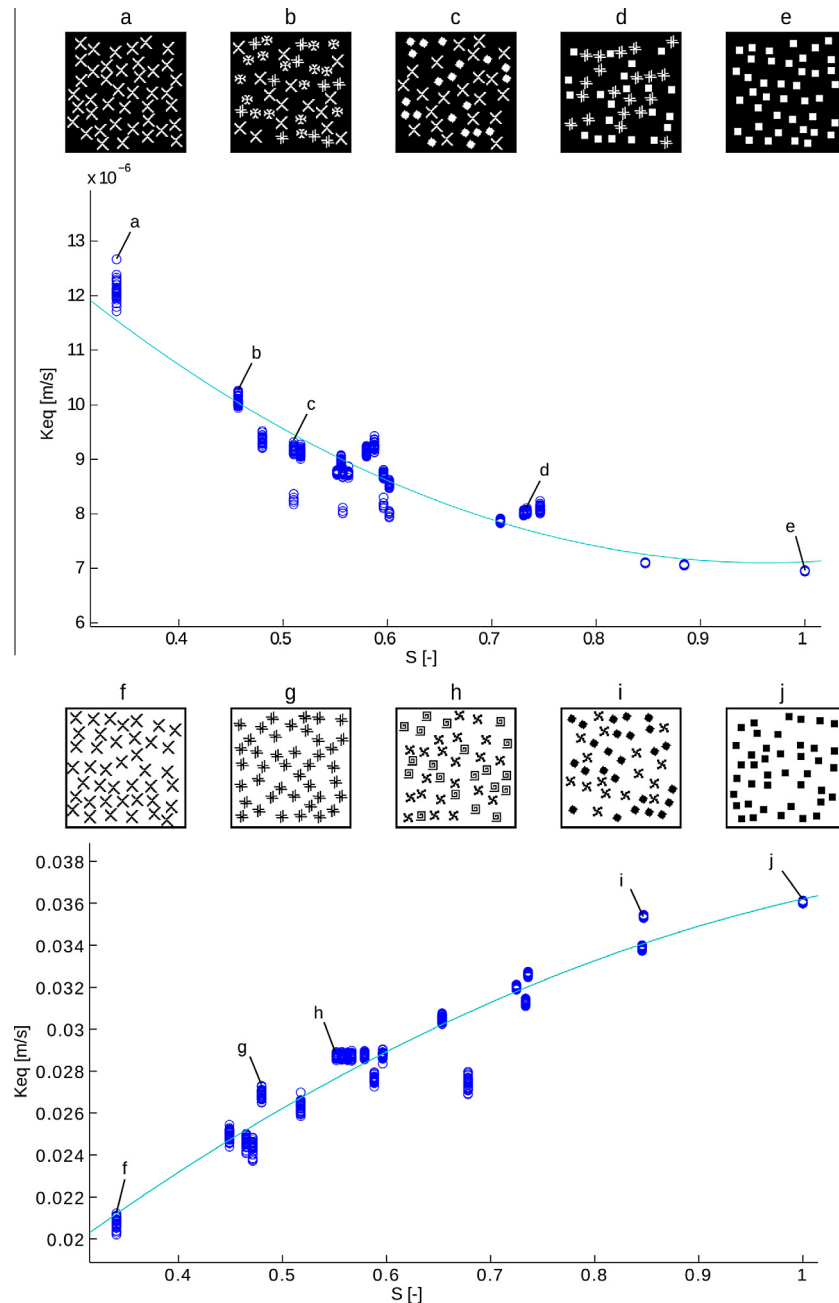
Fig. 3. Test 2, correlation between S and K_{eq} (geometric mean of x and y components). S is computed on HP inclusions (top) and on LP inclusions (bottom) respectively.
