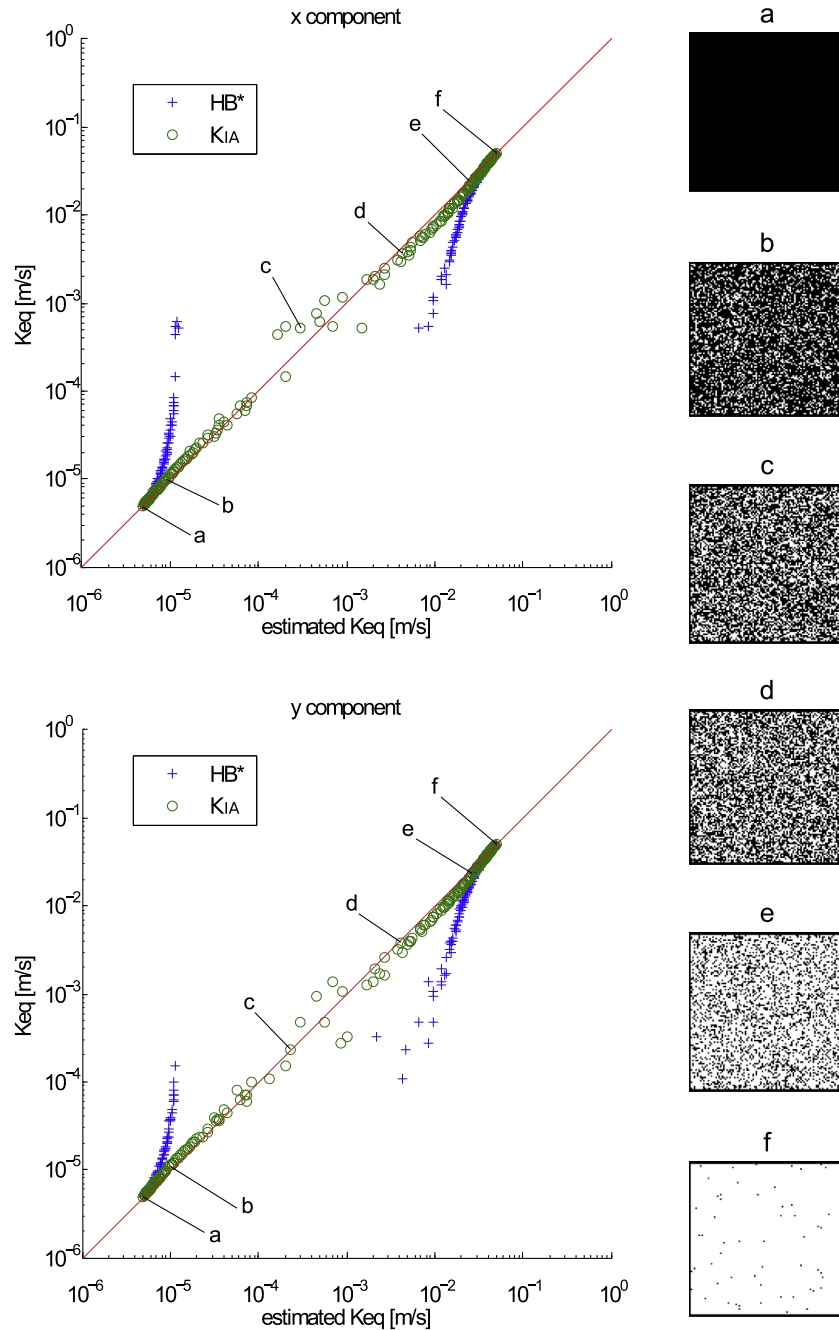
Fig. 5. Test 3, scatter-plot of the reference K_{eq} values as a function of the estimated ones, using the K_{IA} model and the HB^* model. The bisector line indicates the exact estimation. Some examples of the fields are shown on the right, with link to the corresponding data.
