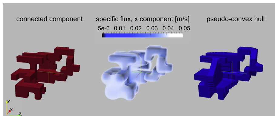
Fig. 9. 3D image of a LP inclusion surrounded by a HP matrix (non-visible). The pseudo-convex hull transformation Pconv(LP, x) and the specific flux x -component v_x are shown. The main flow direction is x . For a matter of visibility, regions presenting v_x > 0.04 (m/s) (undisturbed HP matrix) are omitted from the flow field image.
