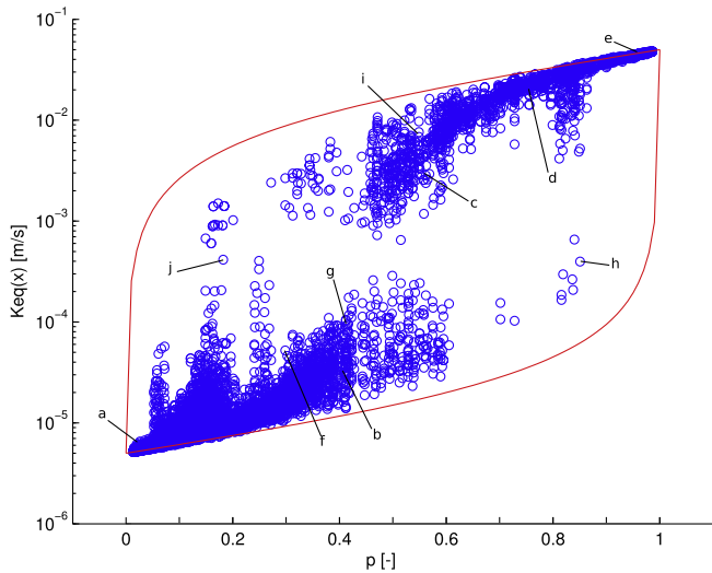
Fig. 6. Test 4, scatter-plot of the x component of K_{eq} as a function of p (proportion of the more conductive hydrofacies). The two curves represent the HS bounds. The alphabetical references correspond to the fields in Fig. 7.
