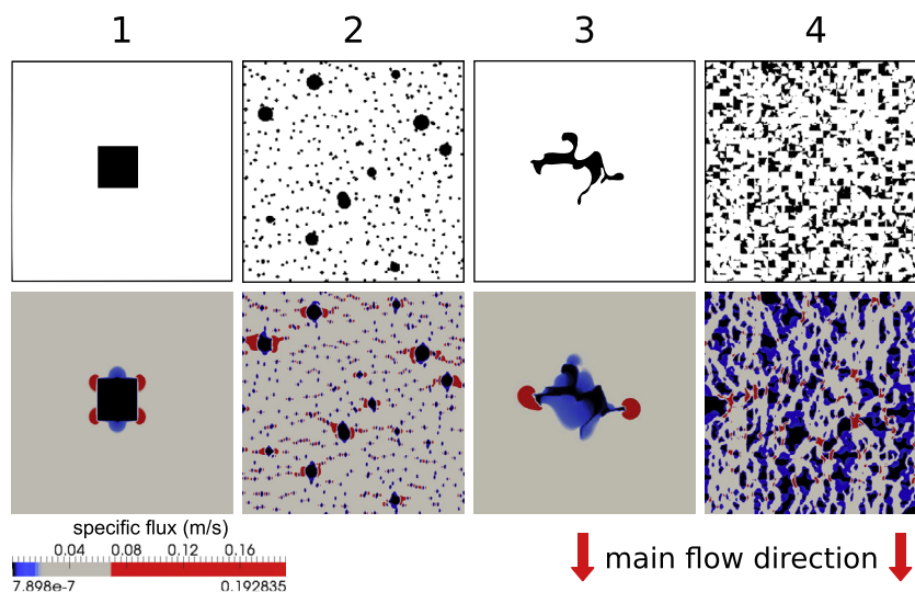
Fig. 1. Example of binary distributions with non conductive inclusions: with convex (1) and (2) and articulated (3) and (4) shapes. Below: the respective specific flux magnitude field with the main flow directed from top to bottom.
