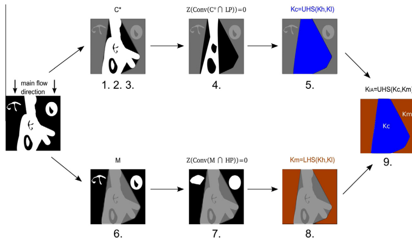
Fig. 4. Schematic illustration of the K_{IA} algorithm, the images show the result of each step, indicated by the corresponding number. The gray shading indicates parts that are not considered.
