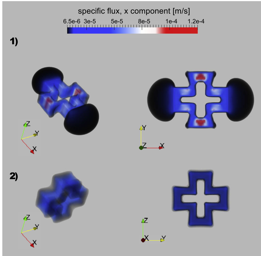
Fig. 10. 3D image of a cross-shaped-torus HP inclusion surrounded by a LP matrix (non-visible), its minor axis being parallel to: (1) the z direction and (2) the x direction. In both cases, the specific flux x -component v_x is shown. The main flow direction is x . For a matter of visibility, regions presenting v_x < 6.5 \times 10^{-6} (m/s) (undisturbed LP matrix) are omitted from the flow field image.
