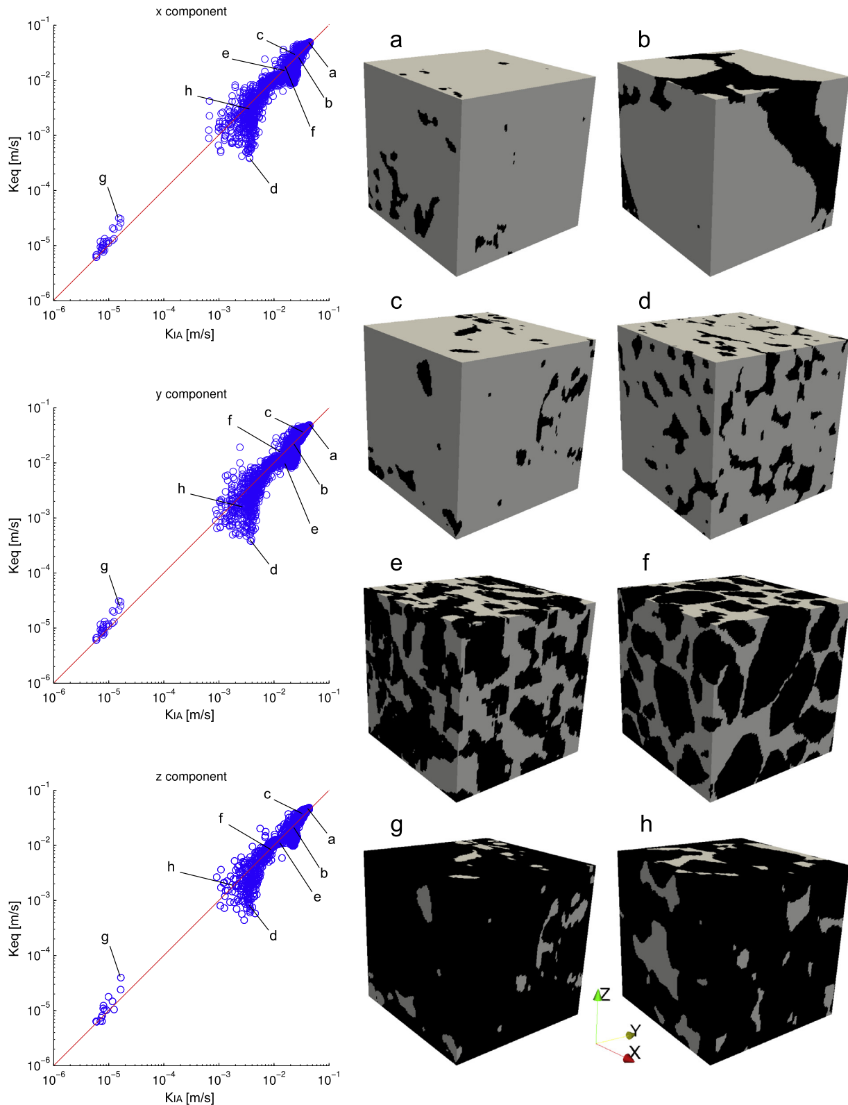
Fig. 12. Test 5, scatter-plot of the reference K_{eq} values as a function of the estimated ones, using the K_{IA} model. The bisector line indicates the exact estimation. Some examples of the fields are shown on the right.
