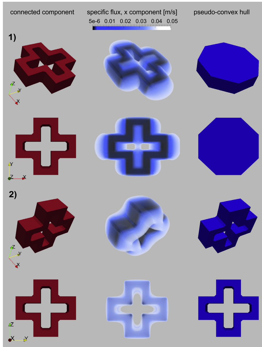
Fig. 8. 3D image of a cross-shaped-torus LP inclusion surrounded by a HP matrix (non-visible), its minor axis being parallel to: (1) the z direction and (2) the x direction. In both cases, the pseudo-convex hull transformation Pconv(LP, x) and the specific flux x -component v_x are shown. The main flow direction is x . For a matter of visibility, regions presenting v_x > 0.04 (m/s) (undisturbed HP matrix) are omitted from the flow field image.
