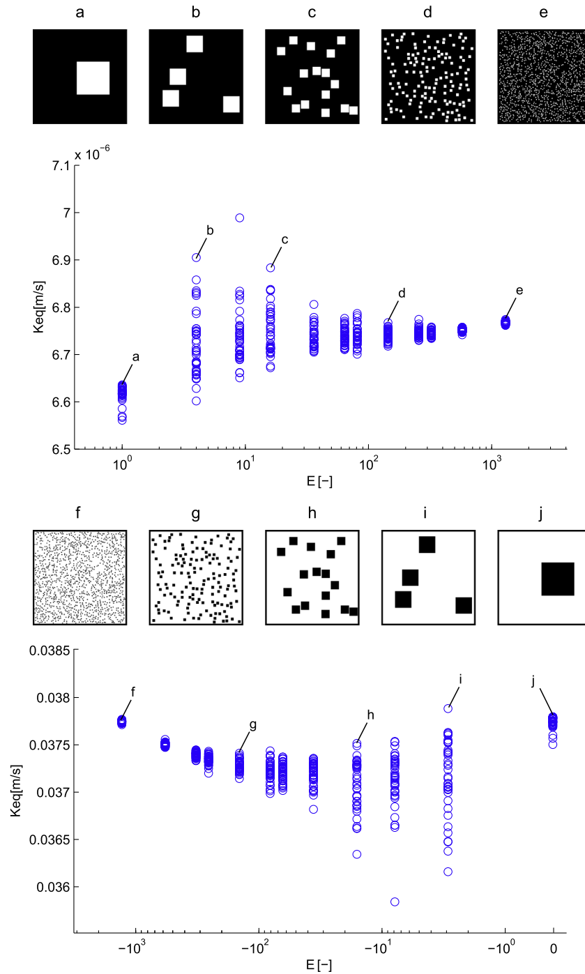
Fig. 2. Test 1, correlation between E (computed on HP) and K_{eq} (geometric mean of x and y components): HP inclusions in a LP matrix (top), HP matrix presenting LP inclusions (bottom). A hybrid log/linear scale is adopted in order to show E = 0 .
