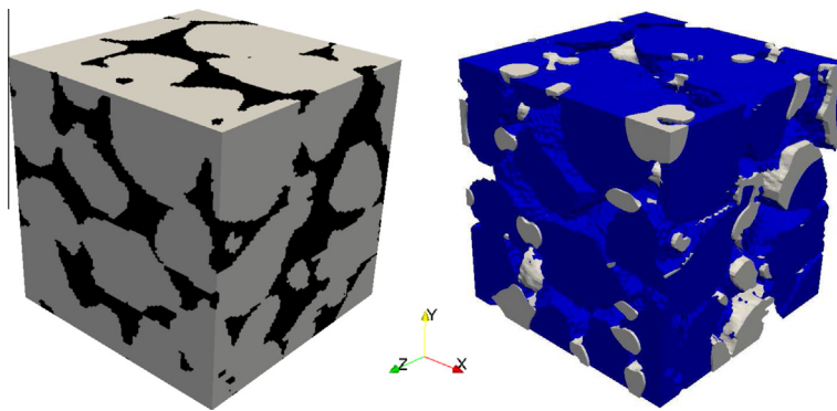
Fig. 11. Example of a 3D binary field presenting a large infinite cluster: LP (black) and HP (white) materials distributions on the left, HP material (blue) and higher velocity regions (gray) on the right, obtained from a flow simulation along the x direction and isolating the regions with v_x \geq 0.05 (m/s). (For interpretation of the references to color in this figure legend, the reader is referred to the web version of this article.)
