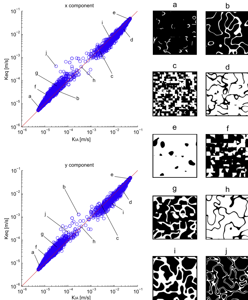
Fig. 7. Test 4, scatter-plot of the reference K_{eq} values as a function of the estimated ones, using the K_{IA} model. The bisector line indicates the exact estimation. Some examples of the fields are shown on the right, with link to the corresponding data.
