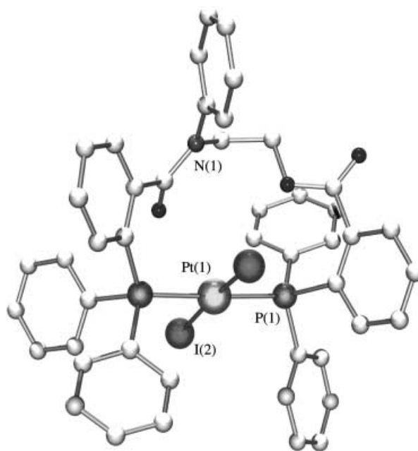
Figure 3. Molecular structure of 18 . Selected bond lengths [Å] and angles [°]: \text{Pt}(1)-\text{P}(1) 2.313(9), \text{Pt}(1)-\text{P}(2) 2.335(9), \text{Pt}(1)-\text{I}(1) 2.610(5), \text{Pt}(1)-\text{I}(2) 2.615(5); \text{P}(1)-\text{Pt}(1)-\text{P}(2) 178.40(4), \text{P}(1)-\text{Pt}(1)-\text{I}(1) 93.52(3), \text{P}(1)-\text{Pt}(1)-\text{I}(2) 89.29(3), \text{P}(2)-\text{Pt}(1)-\text{I}(2) 86.05(3), \text{P}(2)-\text{Pt}(1)-\text{I}(2) 91.30(3), \text{I}(1)-\text{Pt}(1)-\text{I}(2) 173.22(10).
