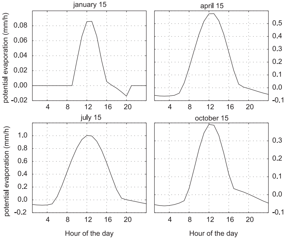
Fig. 2. Example of calculated hourly evaporation for 4 typical days in winter, spring, summer and fall. Note that the negative evaporation corresponds to condensation.
