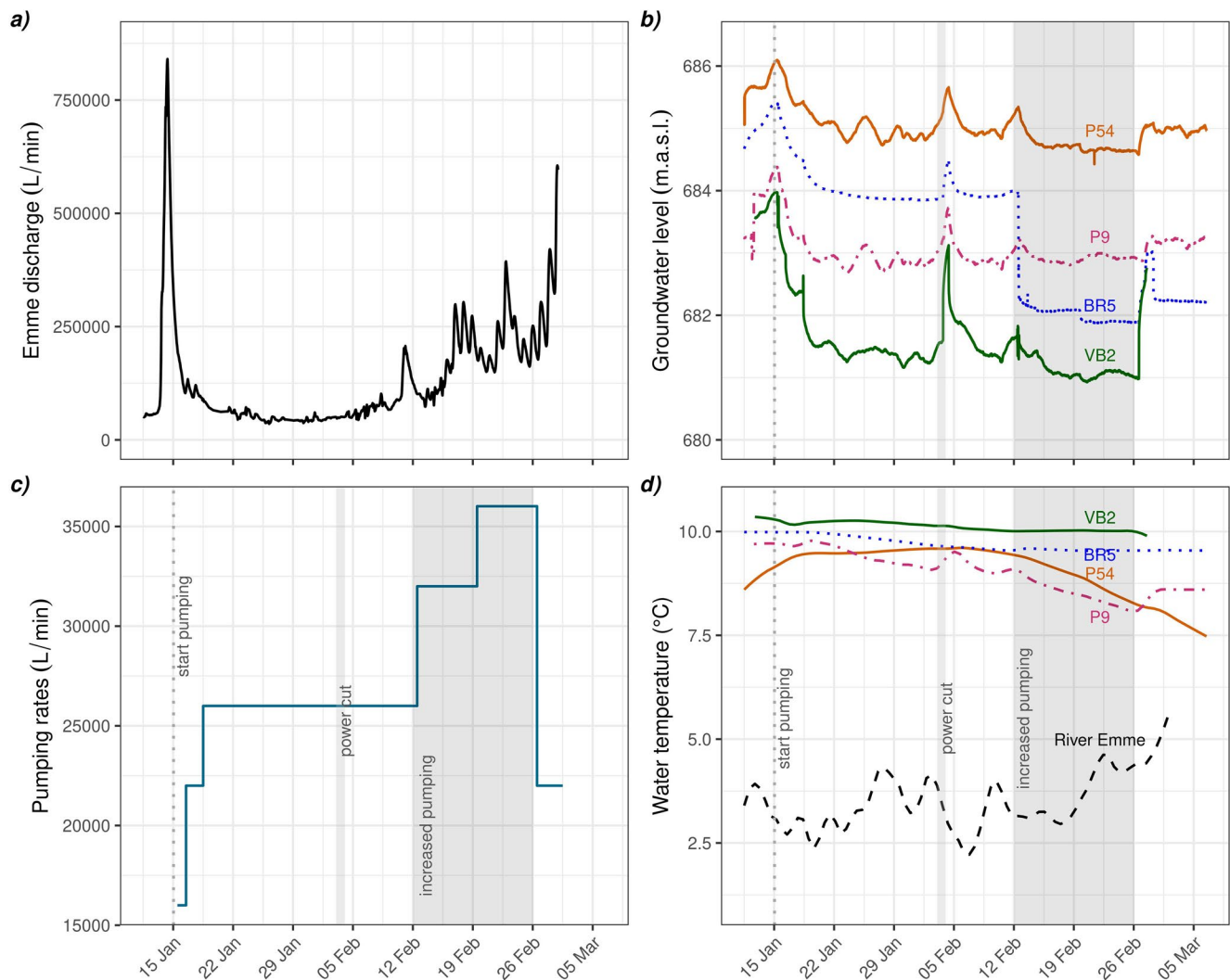
Figure 2. Prevailing conditions during the experiment: (a) the discharge of the Emme (recorded at Heidebühl-Eggiwil ~8 km upstream of the study site), (b) groundwater levels of P54 (orange), VB2 (green), BR5 (dotted, blue) and P9 (dashed, magenta), (c) the total sum of groundwater pumped and (d) water temperatures of P54, VB2, BR5, P9 and the river Emme (dashed, black). The dark gray segment indicates the period of increased pumping (February 12–26). Light gray bands indicate an electric power cut occurring at the study site, which caused a shutdown of all wells from February 3, 6:30 p.m., to the following morning at 10 a.m.
