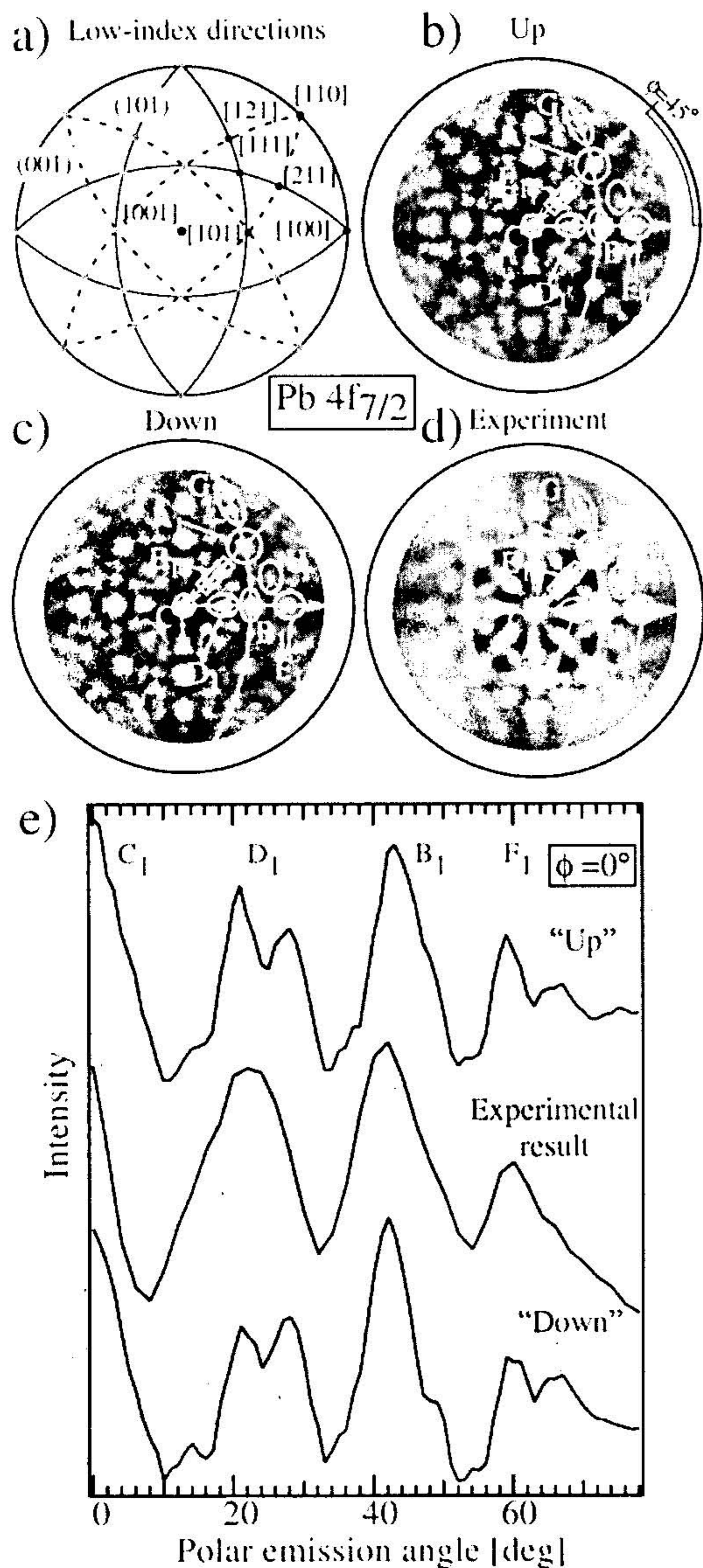
Fig. 4. MgK \alpha excited Pb 4f 7/2 photoelectrons at E_{kin} = 1115.5 eV. (a) Stereographic projection of major directions (dots) and low-index planes (continuous lines correspond to dominant high-density planes \{101\} , dashed lines correspond to minor high-density planes \{\bar{1}11\} ). Simulated diffractograms for PTO (b) “up” and (c) “down” cases. (d) Experimental result for a c -axis oriented PTO 60 Å-thin film. (e) Polar cuts at \phi = 0^\circ for the two simulated states and the experimental case.
