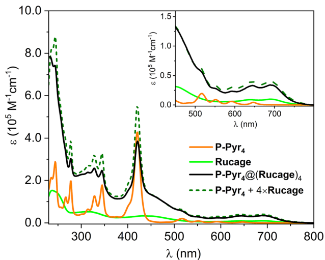
Fig. 4 Absorption spectra of P-Pyr 4 @(Rucage) 4 and its respective models P-Pyr 4 and Rucage in DCM. The weighted sum of the spectra of the models is also reported. Inset: magnification of the 450–800 nm region.
