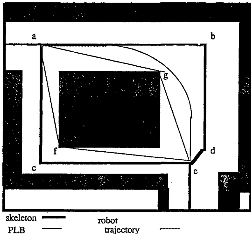
Figure 5.3 Comparing to Barraquand-Latombe
