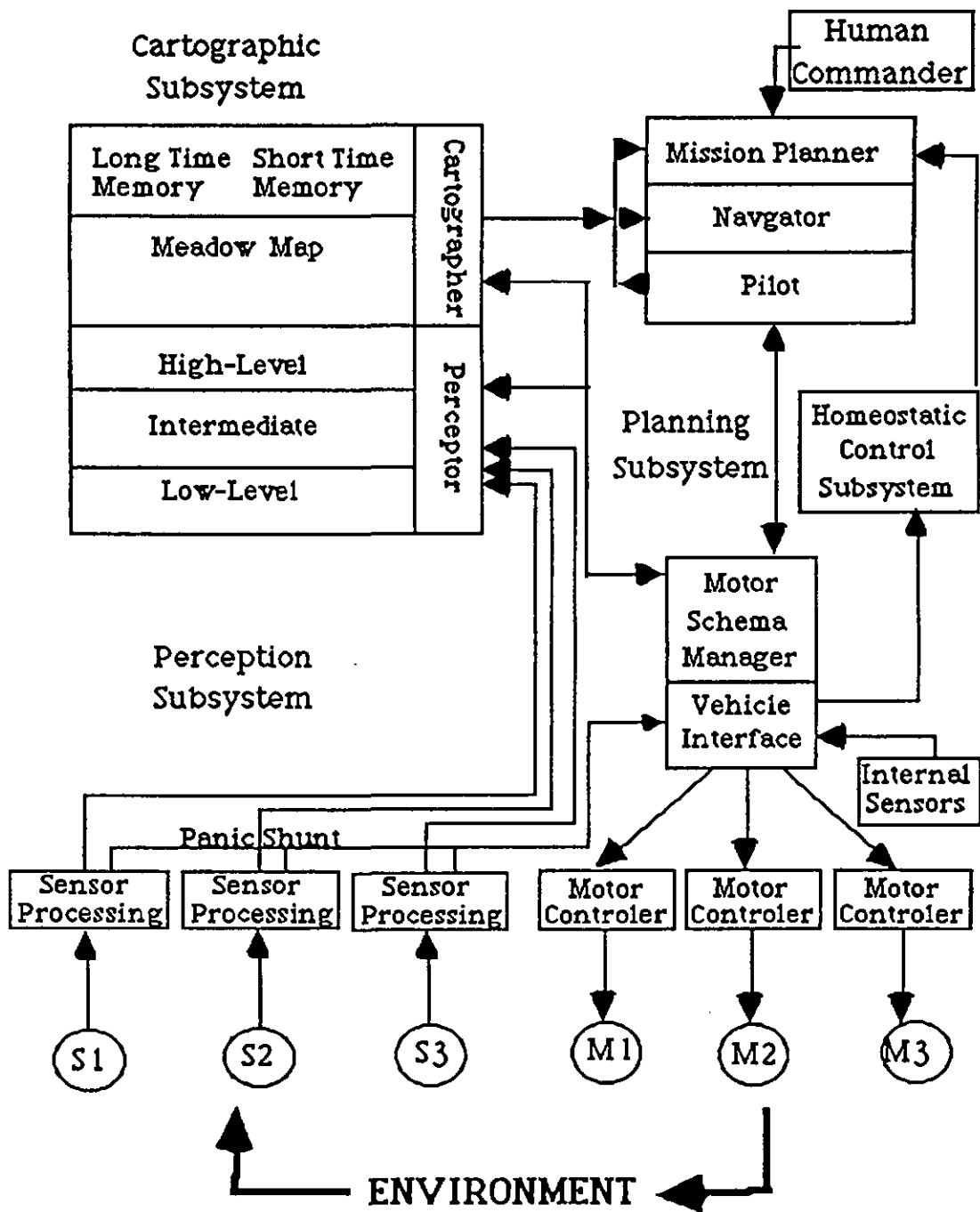
Figure 2.7 The AuRA architecture
