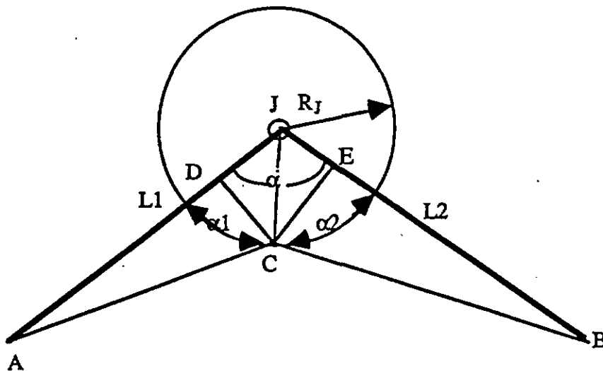
Figure 5.2 Geometric definition
