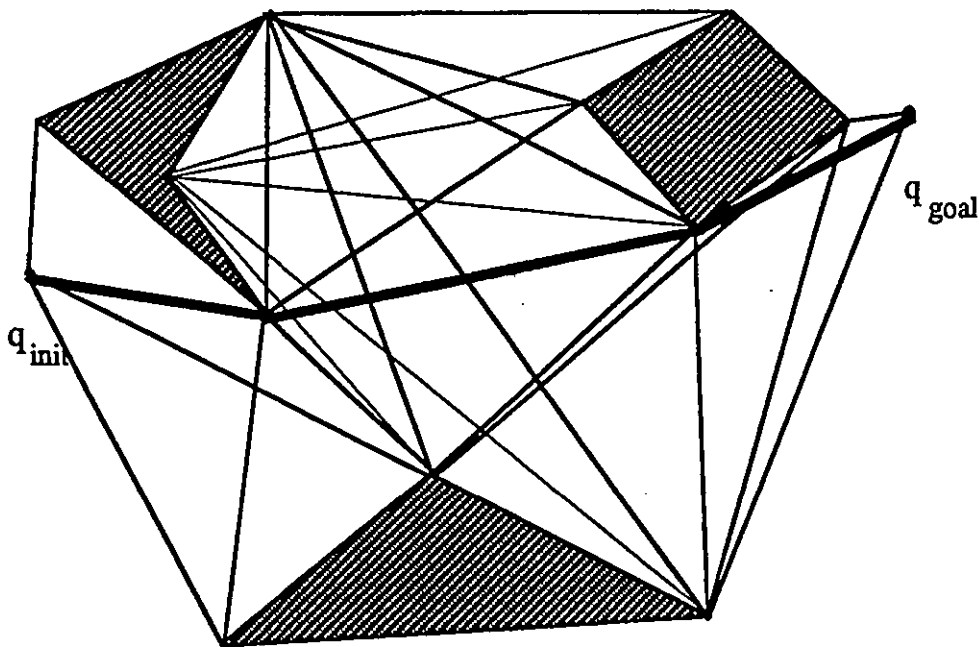
Figure 2.5 Visibility graph. The lines from the concave vertex are broken. The calculated path in bold lines
