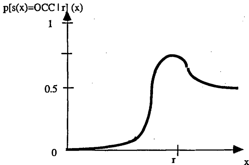
Figure 2.4 occupancy probability profile for real sensor
