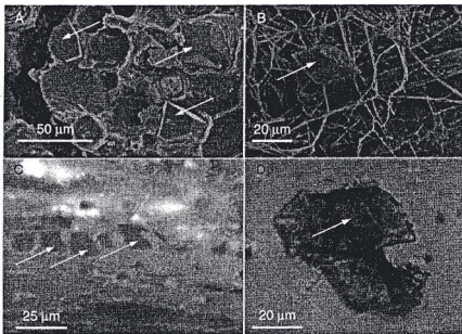
Fig. 12.2. (A) Scanning electron micrograph showing euhedral crystals (arrows) of COD (calcium oxalate dihydrate or weddellite); the other part of the image is mainly cellulose. (B) COD crystal observed with scanning electron microscope. The crystal (arrow) is surrounded by fungi decaying iroko wood whose cellulose fibrous structure is still observable. (C) Ultraviolet-fluorescent light microphotograph of a cross-section inside decaying wood. Between the wood fibres, a chain of dark euhedral crystals of COD has almost been freed in the medium. (D) View with optical binoculars of free crystals of COD inside a soil aggregate. The shape (habitus) of the crystal shown with the arrow is exactly the same as the one of the crystals shown in B.
