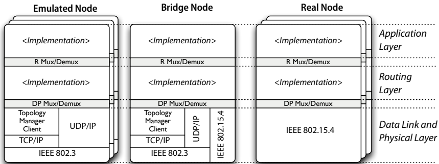
Fig. 2. Layered View of the Software Architecture
