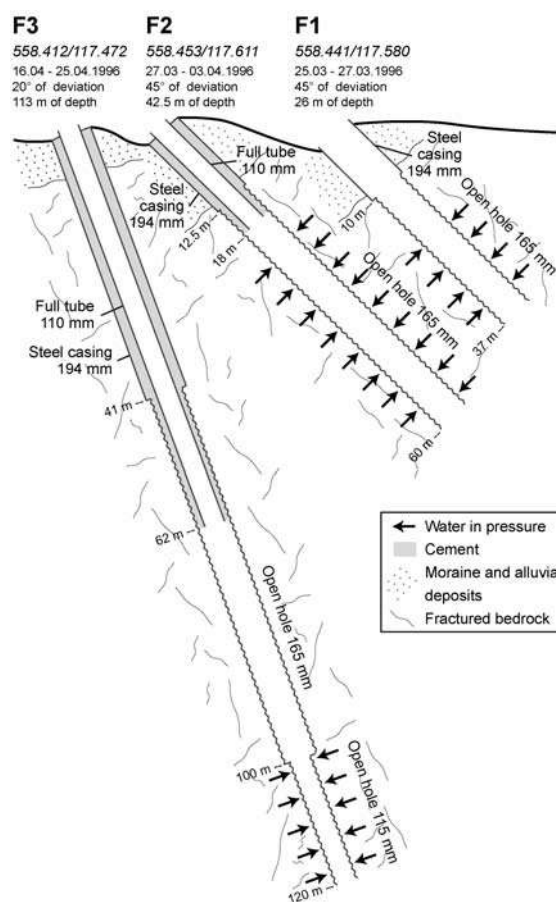
Figure 12.5: Characteristics of the three boreholes in the Val d'Illez modified from Bianchetti (1996). Locations of wells are given in Fig. 12.4.
