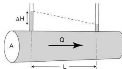
Figure 2.25: Darcy experiment.
