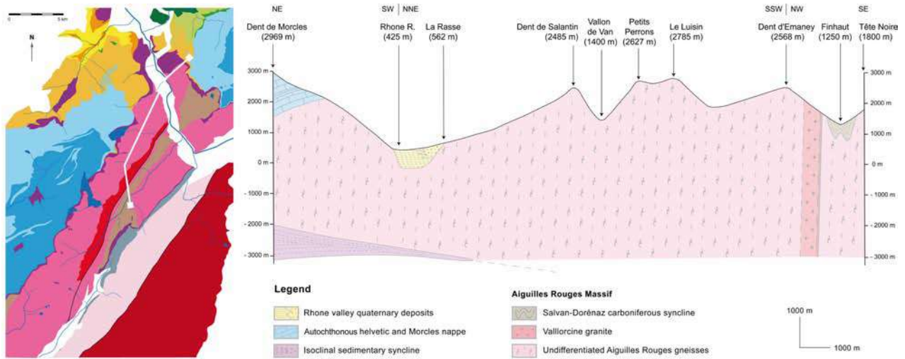
Figure 6.1: Geological cross section of the two-dimensional model for flow and heat transport in the Aiguilles Rouges crystalline Massif. This cross section has two small changes of directions for reason of convenience and to cross the Vallorcine granite (shear zone) which has the same general orientation as the gneiss. The geological map and its legend are visible in Figure 4.1.
