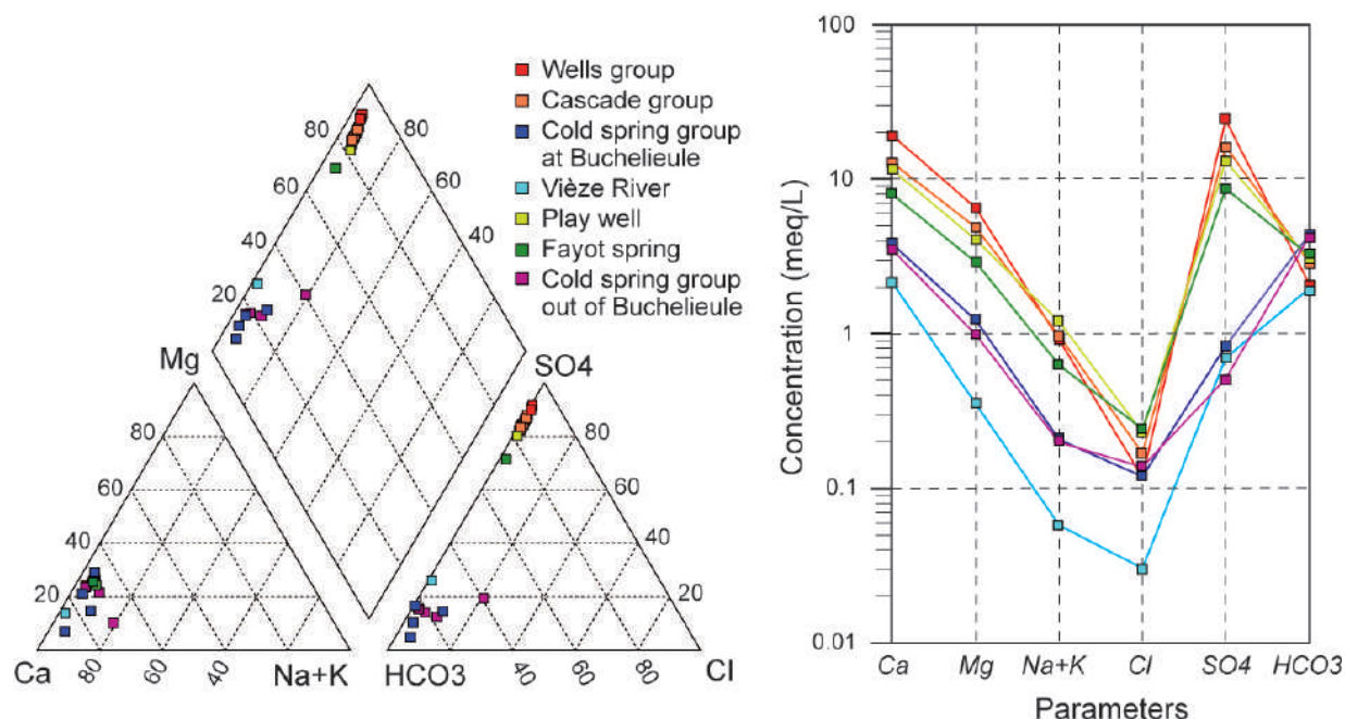
Figure 14.1: Major elements concentration plots (Piper and modified Shoeller diagrams) for groundwaters of the Val d'Illez area with data collected during the new sampling campaign (see data in appendix D). Locations of the samples are shown in Figure 12.3.
