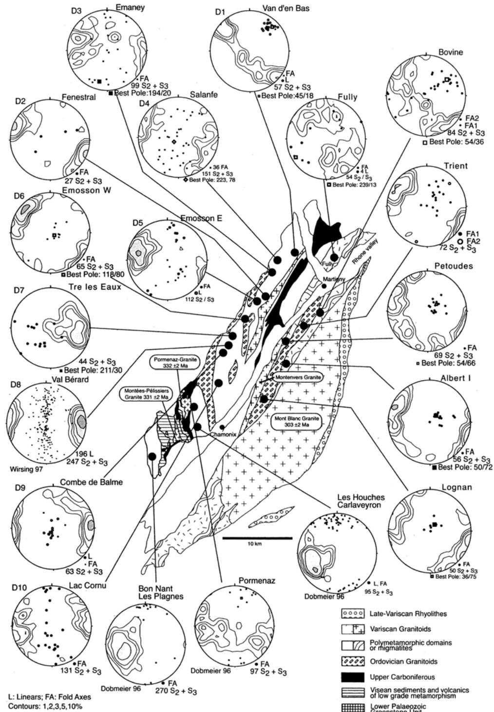
Figure 4.3: Distribution of Late Variscan structures in the polymetamorphic Aiguilles Rouges and Mont Blanc basements. Statistic of dominant orientations of composite surfaces S 2 /S 3 , lineations and fold axes (from Von Raumer and Bussy 2004).
