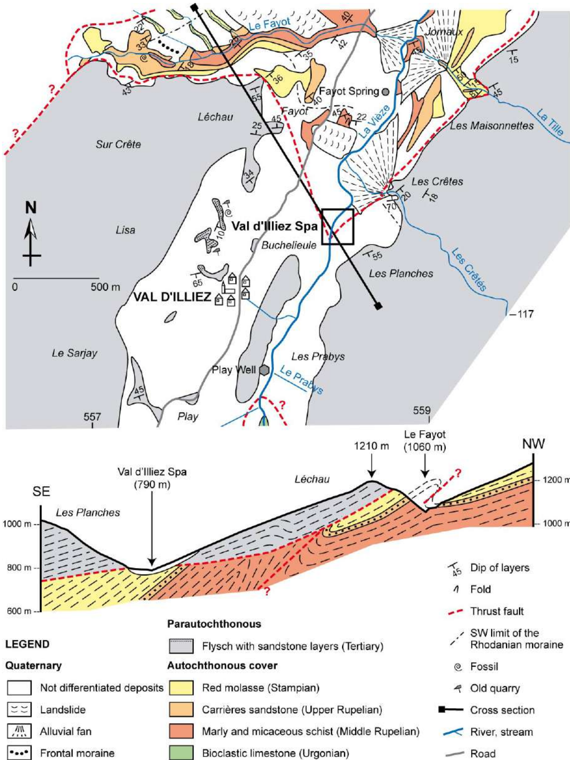
Figure 13.6: Local geological setting of the Val d'Illeiz area (modified from Schroeder and Ducloz 1955).
