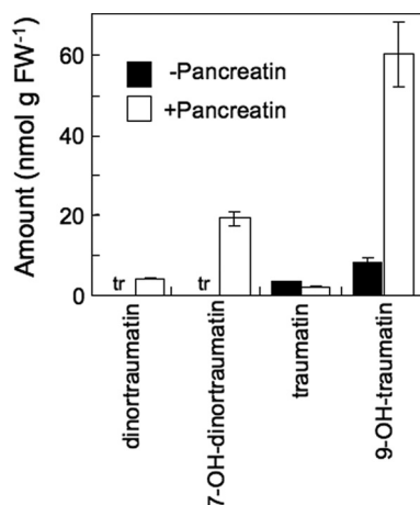
FIGURE 2. Amounts of free and esterified traumatins and its derivatives in leaves of Arabidopsis (No-0). Crude lipids prepared from disrupted Arabidopsis (No-0) leaves were treated with pancreatin or left untreated and then analyzed by LC-MS/MS. In intact leaves, the amounts of free and esterified traumatins and its derivatives were below detection limits. tr , trace. Mean values \pm S.E. (error bars) are shown ( n = 3 ).
