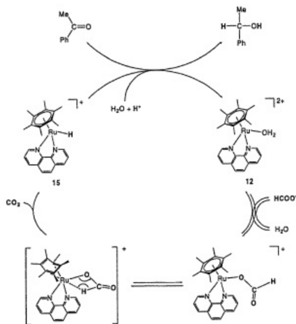
Scheme 1. Postulated catalytic cycle according to Ogo et al. [17].
