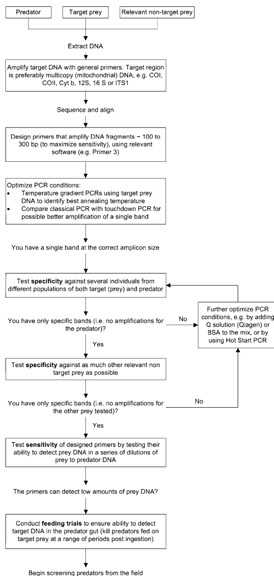
Fig. 1 Basic procedure to design and test primers for use as molecular markers for intraguild predation studies under field conditions. Adapted from King et al. (2008). For further details, see main text or King et al. (2008)
