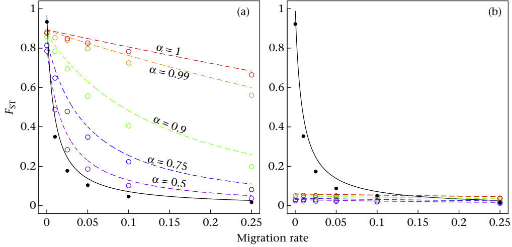
Figure 2. Population structure ( F_{ST} ) in cultural (dashed lines; open circles) and genetic traits (solid lines; filled circles) under low (a; \mu = 0.001 ) and high (b; \mu = 0.1 ) rates of cultural innovation with different probabilities of learning from females ( \alpha ), when only males migrate ( m_f = 0 ); that is, we used the average F_{ST} given by equation (2) over the F_{ij} 's given by equation (A7) for the cultural model and the same average of the sex-specific identities in a diploid genetic model (e.g. Gandon 1999). Lines show analytical results, points show simulation results for a population with a finite number n_d of groups. In all cases, the rate of social learning is set to \beta = 1 - \mu so that the mean frequency of the cultural trait is \rho \approx 0.5 . Parameters for individual-based simulations are: genetic mutation rate \nu_G = 10^{-4} , number of groups n_d = 10 , N_m = N_f = 30 , number of cultural and genetic loci l_C = l_G = 5 . Genetic loci are diallelic, whereas the presence–absence model is a two-state model; we note that, while similar, the transition probabilities due to mutation/innovation in these two models are not exactly equivalent.
