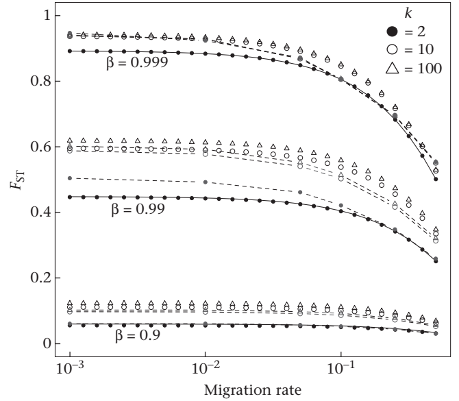
Figure 4. F_{ST} in cultural traits as a function of male migration under the analytical presence-absence model (solid lines without points), analytical k -variants model (points without lines) and in simulations combining presence-absence and k -variants models (points with dashed lines). For the presence-absence model and the simulations, the rates of social learning and innovation are scaled such that \mu = v = 1 - \beta , so that approximately half of the individuals carry cultural traits. For the analytical k -variants model, in all cases \beta = 1 , but the values of \mu and v correspond to those used for the simulations. In all cases, only males migrate and social learning is modelled on females. Measures of F_{ST} are averaged over sex-specific structuring indexes from equation (5) for the presence-absence model and equation (8) for the k -variant model, with p_f = 1/N_f , N_m = N_f = 30 . Other parameters are as in Fig. 2, but n_d = 50 .
