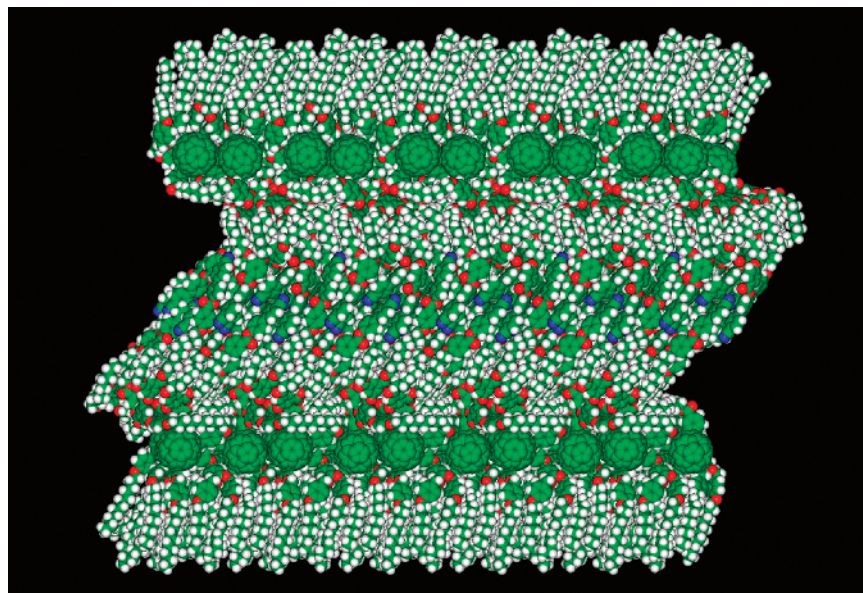
Figure 1. Postulated supramolecular organization of 4 obtained by molecular dynamics. Compounds 5 and 6 gave similar results.
