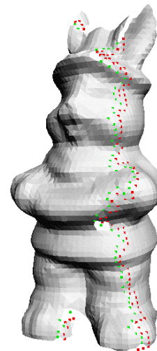
Figure 7: Fusion result
