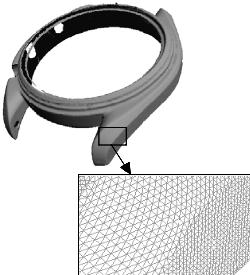
Figure 9: High resolution model of a watch frame
