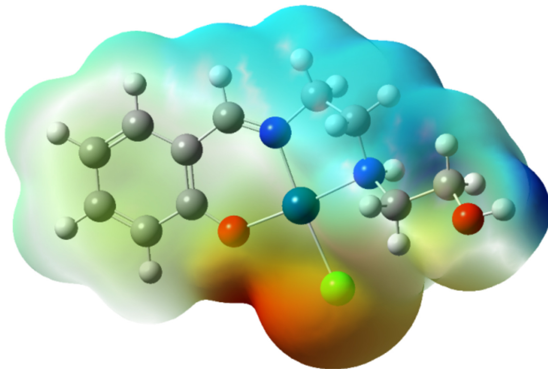
Fig. 3. Molecular electrostatic potential map of [\text{Pd}(\text{L})\text{Cl}] .
