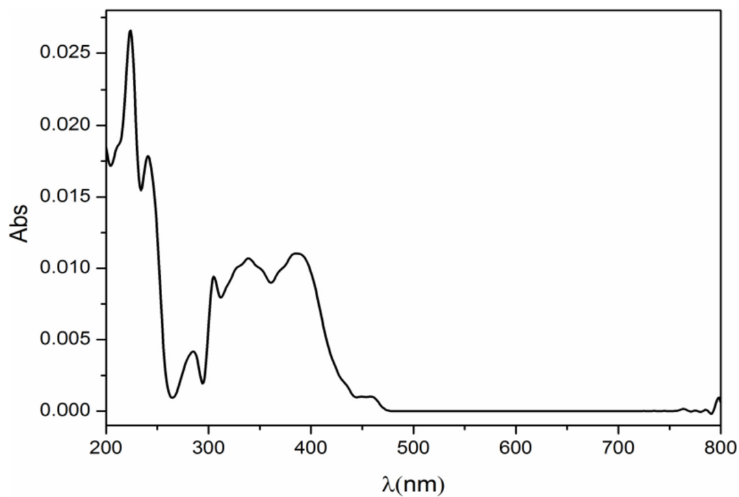
Fig. 4. Experimental UV–Vis spectrum of [\text{Pd}(\text{L})\text{Cl}] in ethanol.
