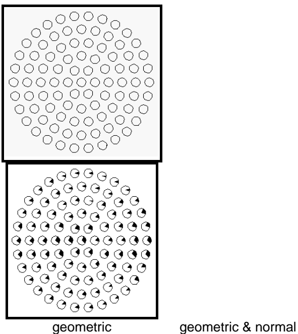
Fig. 3. SIC maps of experiments b
