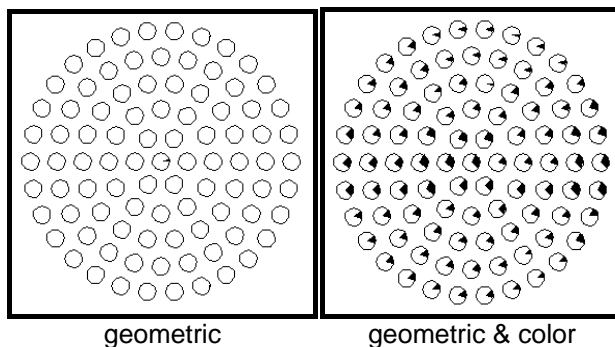
Fig. 4. SIC maps of experiments c
