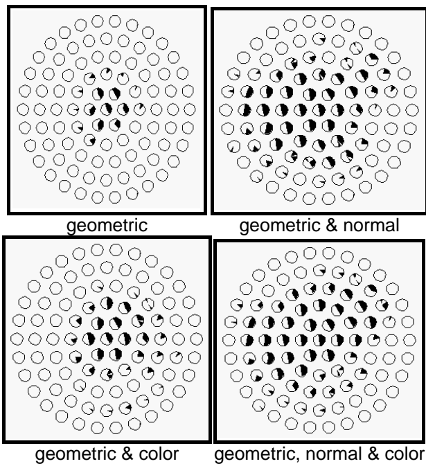
Fig. 2. SIC maps of experiment a
