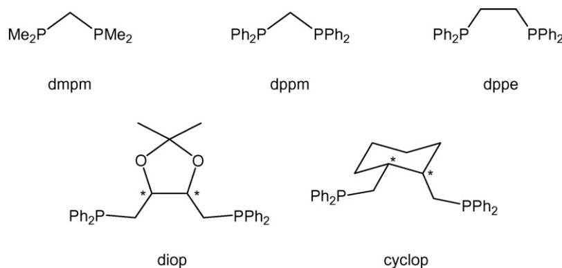
Scheme 3. Schematic representations of non-chiral and chiral diphosphine (diphos) ligands of the type R_2P \cap PR_2 .
