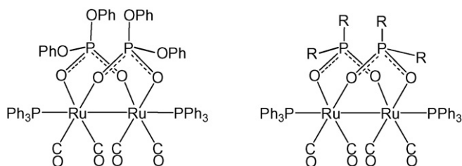
Fig. 22. Phosphato [75] and phosphinito [73,74] complexes based on a diruthenium tetracarbonyl sawhorse structure.
