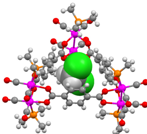
Fig. 37. Molecular structure of [CH 2 Cl 2 ·Ru 6 (CO) 12 (OOCC 6 H 4 COO) 2 (PMe 3 ) 6 ] [120].
