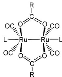
Fig. 3. The sawhorse geometry of \text{Ru}_2(\text{CO})_4(\text{OOCR})_2\text{L}_2 complexes (2 perspectives).
