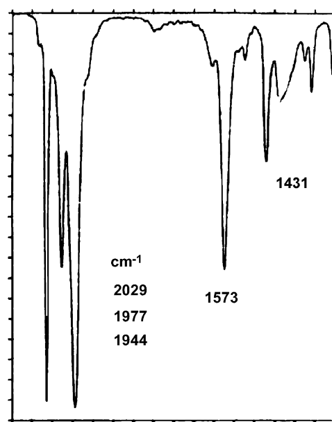
Fig. 9. Infrared spectrum of \text{Ru}_2(\text{CO})_4(\text{OOCeEt})_2(\text{N}_2\text{C}_3\text{H}_4)_2 in \text{CH}_2\text{Cl}_2 [19].
