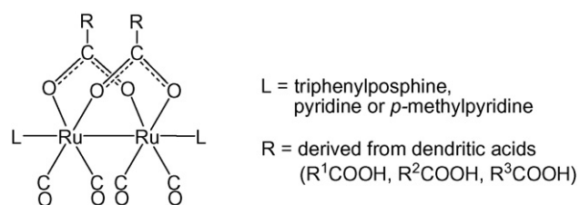
Fig. 30. Mesomorphic \text{Ru}_2(\text{CO})_4(\text{OOCR})_2\text{L}_2 complexes containing mesogenic dendritic substituents in the carboxylato bridges [14].
