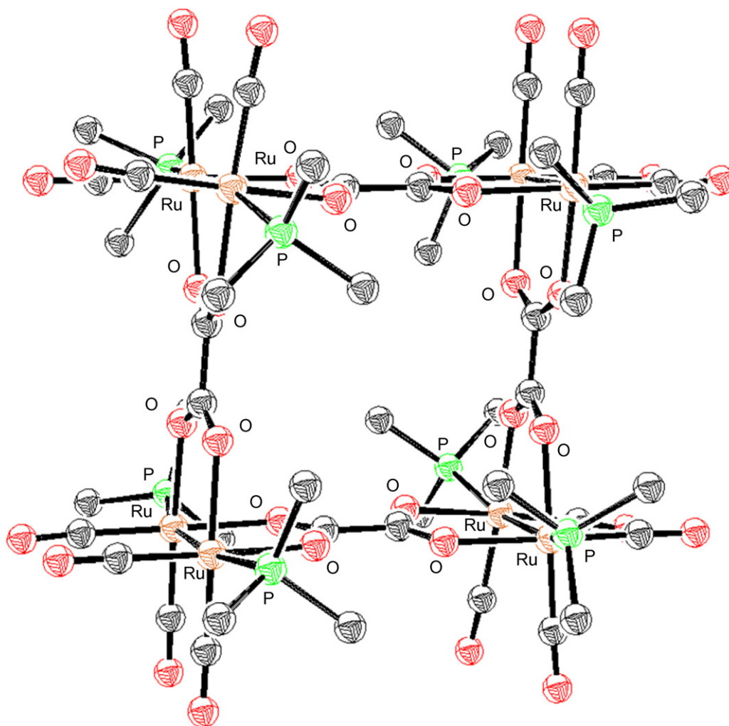
Fig. 38. Molecular structure of Ru 8 (CO) 16 (OOCCOO) 4 (PMe 3 ) 8 [118].
