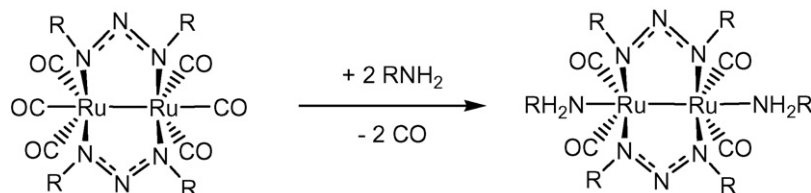
Scheme 7. Triazenido-bridged diruthenium tetracarbonyl sawhorse systems [51].
