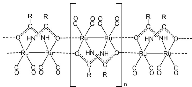
Fig. 11. Proposed structure for the polymers [\text{Ru}_2(\text{CO})_4(\text{OHCR})_2]_n , the connection between the sawhorse units being assured by Ru–O interactions [16].
