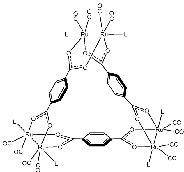
Fig. 36. Molecular triangle arrangement in Ru 6 (CO) 12 (OOCC 6 H 4 COO) 2 L 6 [120].
