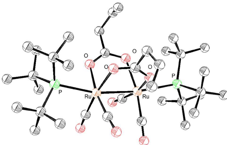
Fig. 1. Molecular structure of \text{Ru}_2(\text{CO})_4(\text{OOCPr}^n)_2(\text{PBu}^t_3)_2 [2].
