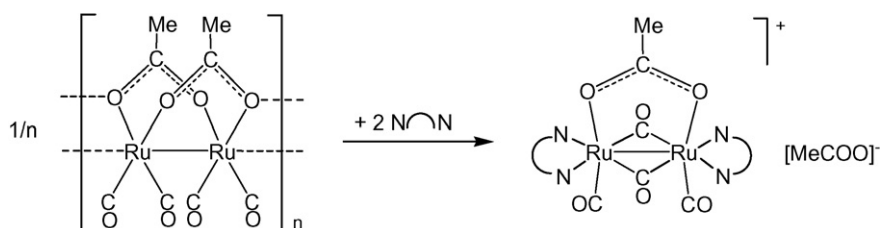
Scheme 4. Reactivity of polymeric carboxylato-bridged diruthenium tetracarbonyl complexes towards aromatic diimes ( N \cap N ) [35–38].
