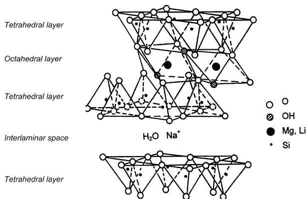
Fig. 1. Structural model according to Grim [12] of sodium hectorite Mg_{5.5}Li_{0.5}Si_8O_{20}(OH)_4 Na \cdot n H_2O , showing the anionic three-layer sheets and the interlaminar space containing sodium cations and water molecules.
