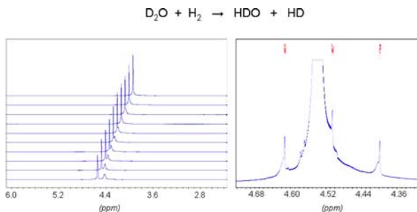
Fig. 4. ^1H NMR spectra of a D_2O suspension of 2 under a H_2 pressure of 100 bar at 50^\circ C . Left-hand figure: Spectral evolution during the formation of 3 , showing the increase of the HDO signal (left) and the rapid decrease of the H_2 signal (right) over a period of 10 min, the time interval being 1 min. Right-hand figure: Spectrum after repressurizing the sample with H_2 (50 bar) at 50^\circ C , showing the triplet signal of HD ( J = 43 Hz) besides the large (central) HDO signal.
