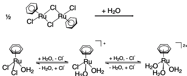
Scheme 1. Hydrolysis of the dinuclear complex [(C_6H_6)RuCl_2]_2 in water to give a mixture of mononuclear benzene ruthenium complexes, the dicationic triaqua complex [(C_6H_6)Ru(H_2O)_3]^{2+} being the major product.
