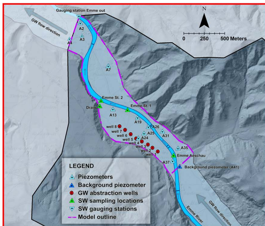
Figure 2. (top) Maps of the Upper Emme catchment and (bottom) a close-up of the GW pumping station on the Ramsei Plain in the lower part of the catchment. In the top image, bright blue colors in the valley bottoms indicate aquifers. The different subcatchments are separated by solid black lines. The three gauging stations that measure the discharge of each subcatchment are indicated by inverted blue triangles.
