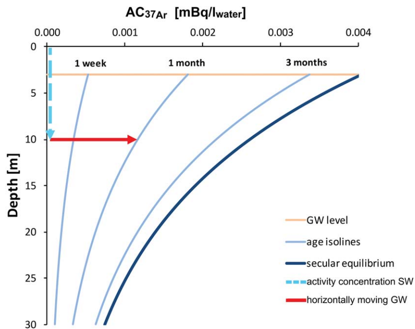
Figure 1. ^{37}\text{Ar} -dating concept. The concept is illustrated for a parcel of SW with a near-zero AC_{37Ar,SW} , that infiltrated rapidly, and which starts moving horizontally in GW at a depth of 10 m. Once in the subsurface, the water parcel starts accumulating ^{37}\text{Ar} . After 110 days, the water parcel reaches the secular equilibrium of ^{37}\text{Ar} , which, at 10 m depth ( AC_{37Ar,eq}(10 \text{ m}) ), would be 0.00268 \text{ mBq/L}_{\text{water}} for an attenuation length of 15.9 m. If the water parcel is sampled before 110 days of residing in the subsurface, for example, after 1 month, the ^{37}\text{Ar} activity concentration can be used to identify the residence time of that water parcel.
