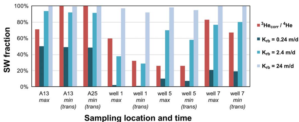
Figure 8. Comparison between the {}^3\text{He}_{\text{corr}}/{}^4\text{He} -based SW fraction and the simulated SW fraction. The max measurements are compared to the steady state max simulations, and the min measurements are compared to the trans simulations.
