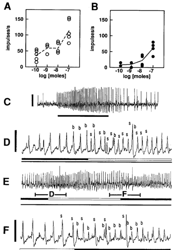
Fig. 7. A–C Response of receptors sensitive to 2-hydroxybenzaldehyde and benzaldehyde in the proximal region VI of the capsule of Haller's organ in A. variegatum . A Dose (moles in stimulus cartridge) of 2-hydroxybenzaldehyde ( n = 5 different ticks) and B dose of benzaldehyde ( n = 4 different ticks) plotted against spike frequency of the responding receptor calculated from the first 200 ms of the response. Trend lines connect mean values. In A and B the response of each receptor increased with increasing doses throughout the range tested. C Representative response of the receptor to 2-hydroxybenzaldehyde at 10^{-9} moles in the stimulus cartridge. D–F Double successive stimulation while recording from a receptor responding to benzaldehyde ( solid horizontal bar ) interrupted for 1 s ( hollow horizontal bar in E ) by stimulation with 2-hydroxybenzaldehyde (both products at 10^{-8} moles in separate stimulus cartridges). A phasic burst in spike frequency of a second excited cell at onset of stimulation with 2-hydroxybenzaldehyde and at restart with benzaldehyde indicated presence of separate receptors ( b and s respectively, in D and F ) for these two products in region VI of the capsule of Haller's organ. D Spike train illustrating response to last 200 ms of stimulation with benzaldehyde and corresponding onset period with 2-hydroxybenzaldehyde. F Spike train resulting from reverse of situation in D , i.e. last 200 ms of stimulation with 2-hydroxybenzaldehyde and restart of stimulation with benzaldehyde. Solid horizontal bar in C and hollow bar in E represent 1 s; vertical bars 1 mV
