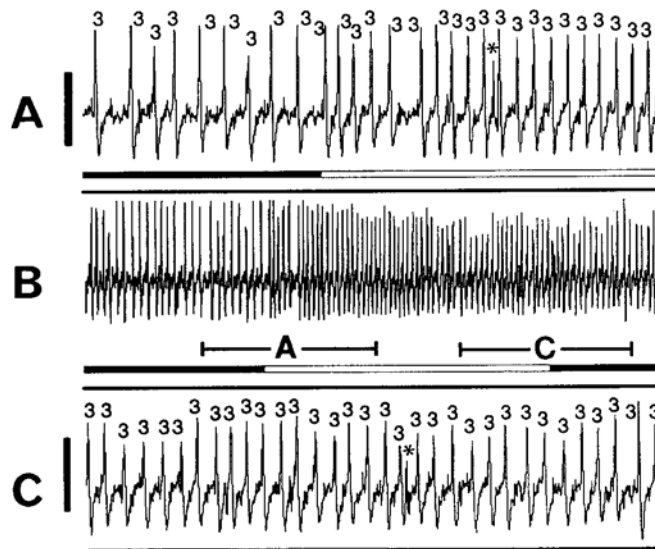
Fig. 9A–C. Response of an olfactory receptor (aldehyde receptor type 3) located within the proximal region VI of the capsule of Haller's organ in a male A. variegatum to the unsaturated aldehydes (E)-2-hexenal and (E)-2-heptenal (each at 10^{-8} moles in the stimulus cartridge). B Double successive stimulation with (E)-2-heptenal (solid bar) interrupted for 1 s by stimulation with (E)-2-hexenal (hollow bar). Absence of a second responding unit at onset of stimulation with (E)-2-hexenal or at restart of stimulation with (E)-2-heptenal indicated that both products activated the same receptor. This receptor type did not respond to short-chain saturated aliphatic aldehydes. A Spike train illustrating response to the last 300 ms of stimulation with (E)-2-heptenal and corresponding period from onset of stimulation with (E)-2-hexenal. C Spike train resulting from reverse of the stimulation in A, i.e. last 300 ms of stimulation with (E)-2-hexenal and restart of stimulation with (E)-2-heptenal. At least one other receptor with a spike of smaller amplitude (star) occurs in these traces. Vertical bars 1 mV
