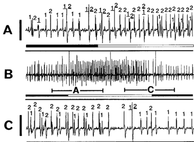
Fig. 8A–C. Response of olfactory receptors located within the proximal region VI of the capsule of Haller's organ in a male A. variegatum to the short-chain aliphatic aldehydes (E)-2-hexenal and hexanal (each at 10^{-8} moles in the stimulus cartridge). B Double successive stimulation with (E)-2-hexenal (solid bar), which stimulated both receptor 1 and receptor 2 weakly, was interrupted for 1 s by stimulation with hexanal (hollow bar) which activated receptor 2 more than (E)-2-hexenal did. Sensitivity of receptor 1 to both aldehydes was approximately the same. A Spike train illustrating response to last 300 ms of stimulation with (E)-2-hexenal and corresponding period from onset of stimulation with hexanal. C Spike train resulting from reverse of the situation in A, i.e. last 300 ms of stimulation with hexanal and restart of stimulation with (E)-2-hexenal. Spikes with underlined numbering are overlapping events; vertical bars 1 mV
