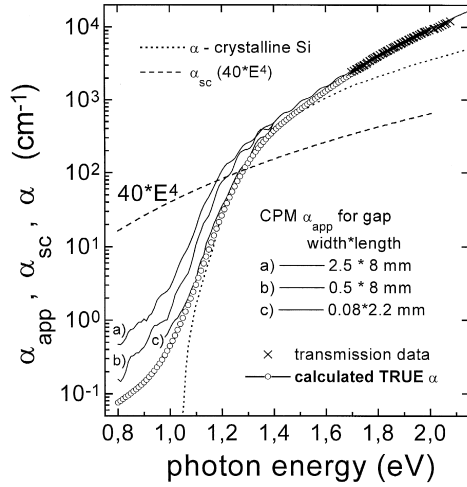
Fig. 4. Absolute CPM spectra \alpha_{app} of a mirror-like \mu c-Si film and ‘true’ \alpha(E) evaluated from all CPM data. Here the \alpha_{app}(E) approaches the \alpha(E) for 80 \mu m spacing between the evaporated electrodes.
