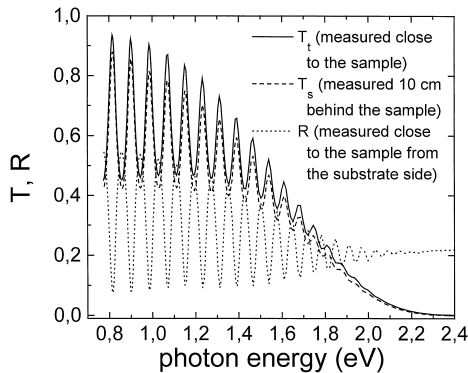
Fig. 1. Transmittance T and reflectance R spectra of a typical textured microcrystalline Si layer, deposited by VHF-GD.
