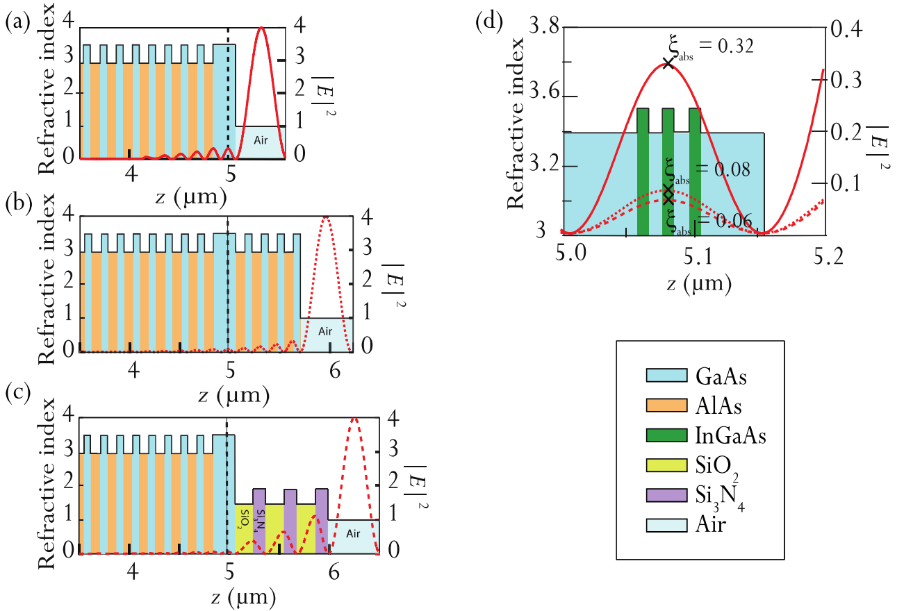
Figure 7. Different SESAM structures used for the damage studies (a) SESAM design with 3 QWs and no topcoating (NTC); (b) same SESAM but with a 4-quarter-wave-pair GaAs/AlAs semiconductor topcoating (SCTC); (c) same SESAM but with a 3-quarter-wave pair \text{SiO}_2/\text{Si}_3\text{N}_4 dielectric topcoating (DTC3); (d) field enhancement in the absorber section.
