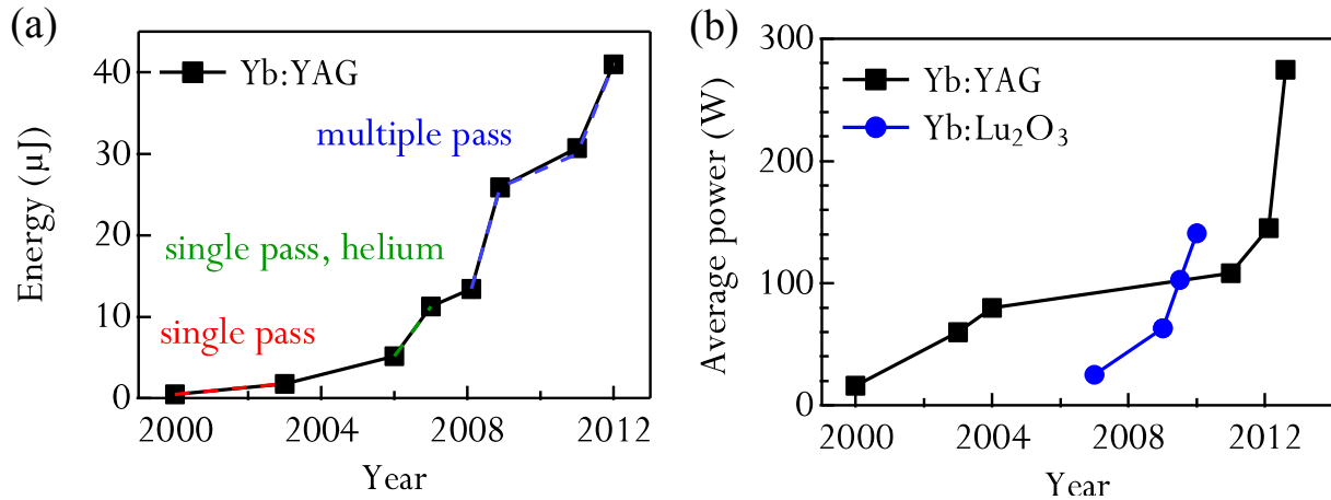
Figure 1. Evolution of pulse energy (a) and average power (b) of ultrafast semiconductor saturable absorber mirrors (SESAM)-modelocked thin-disk laser (TDLs). Most power and energy scaling was achieved using the well-established gain material Yb:YAG, but promising new materials for this application are currently the topic of important research efforts.
