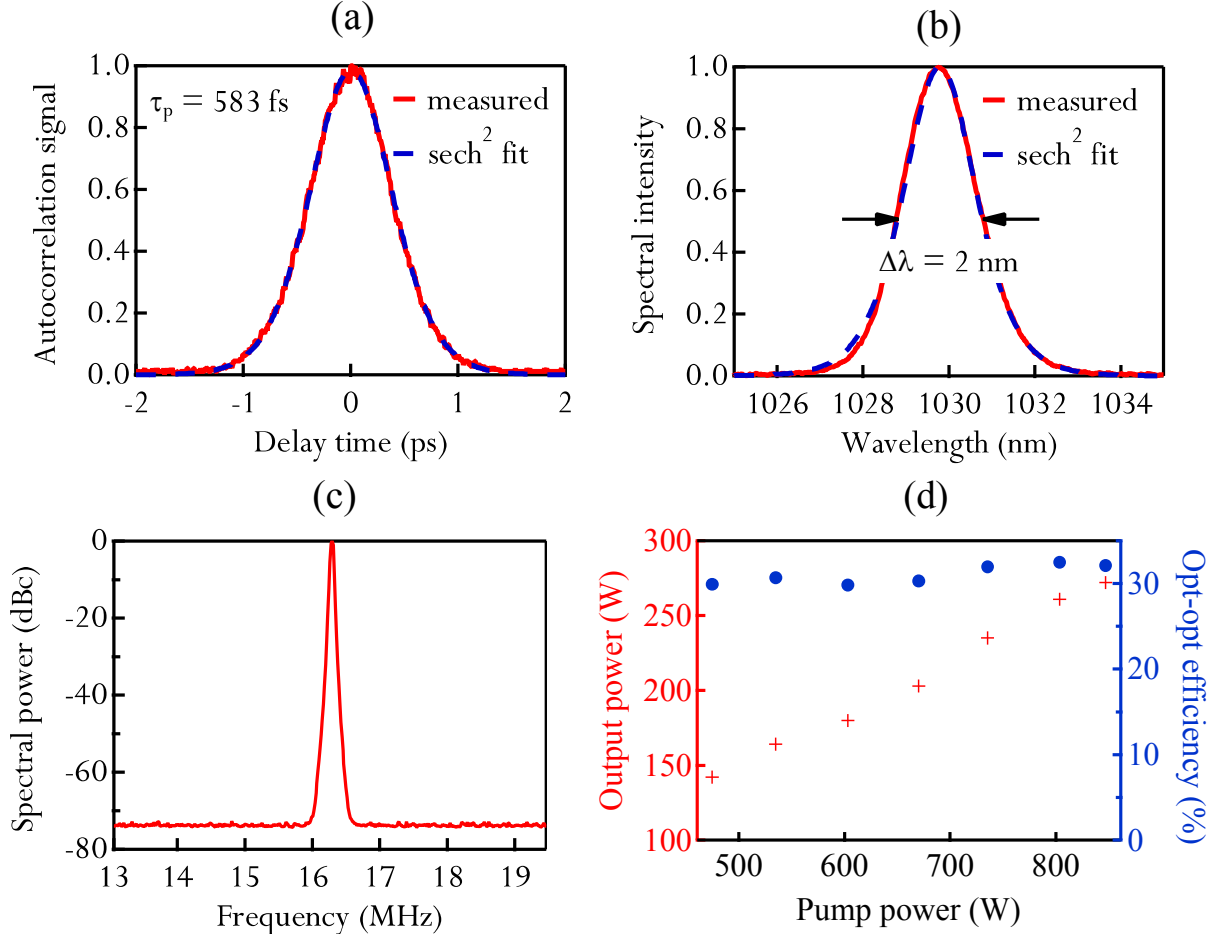
Figure 5. (a) Autocorrelation trace of the pulses at the maximum average output power of 275 W; (b) Optical spectrum of the pulses; (c) Radio frequency spectrum of the pulses, with a resolution bandwidth of 30 kHz; (d) Output power and optical-to-optical efficiency in modelocked operation as a function of pump power. The points before modelocking were not measured in order to avoid damage of intracavity components during the Q-switched modelocking (QML) regime that occurs before modelocked operation.
