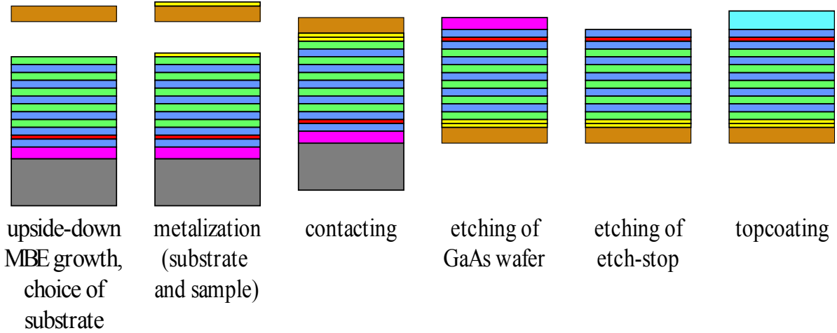
Figure 13. Schematic of the fabrication steps of future generation upside-down high-power SESAMs.
