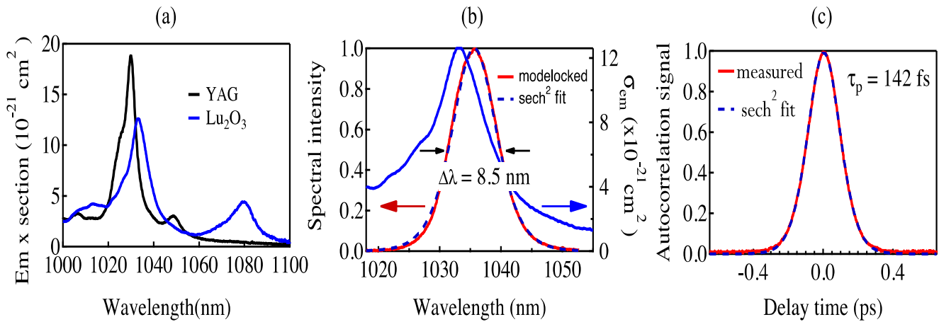
Figure 17. (a) Emission spectrum of Yb:LuO and Yb:YAG. (b) Spectrum of the modelocked laser delivering 142 fs, showing a 8.5 nm-wide (FWHM) modelocked spectrum, together with the 12.5 nm wide emission spectrum of Yb:LuO. The observed red-shift of the modelocked spectrum is due to the low inversion level at which the laser is operated. Strictly speaking, the modelocked spectrum should be compared not to the emission spectrum, but to the exact gain cross section at the inversion level \beta at which the laser operates (see Figure 16). However, different sources of spectrally dependent loss (such as the reflectivity of the different dielectric mirrors in the cavity, or the SESAM) make the precise determination of \beta a challenging task. Therefore, a comparison to the emission spectrum is here more adequate. (c) Autocorrelation trace of the 142 fs pulses obtained at 7 W of average output power.
