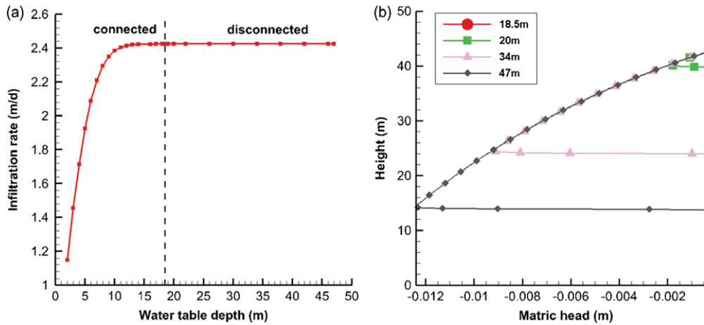
Figure 3. The variation in (a) the infiltration rate through the bottom of the stream and (b) the matric head profile beneath the stream (i.e., at x = 0 m) between the stream bottom and the base of the aquifer for four depths of the RWT. Matric head of 0 m in (b) indicates full saturation.
