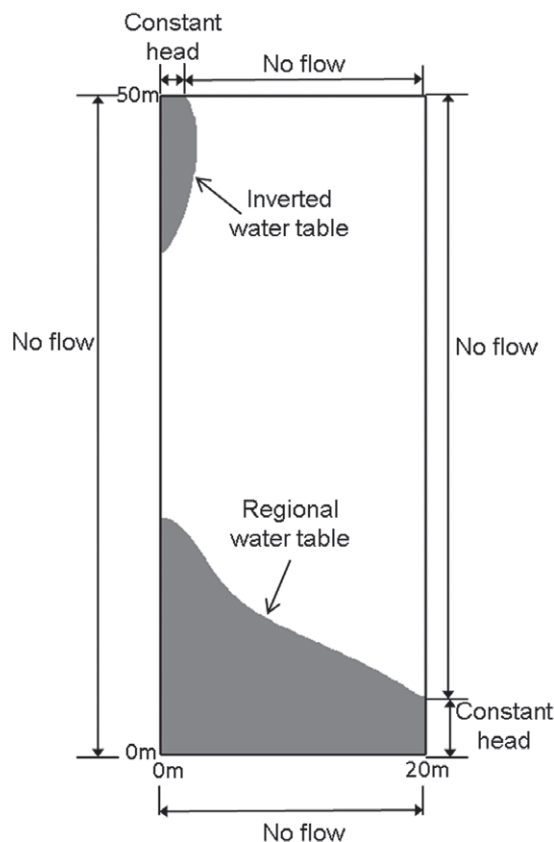
Figure 1. Geometry and boundary conditions of the model domain. The hydraulic head boundary condition in the top left represents the stream. Another hydraulic head boundary condition is placed at the lower part of the right-hand side to represent regional groundwater. All other boundary conditions are no flow.
