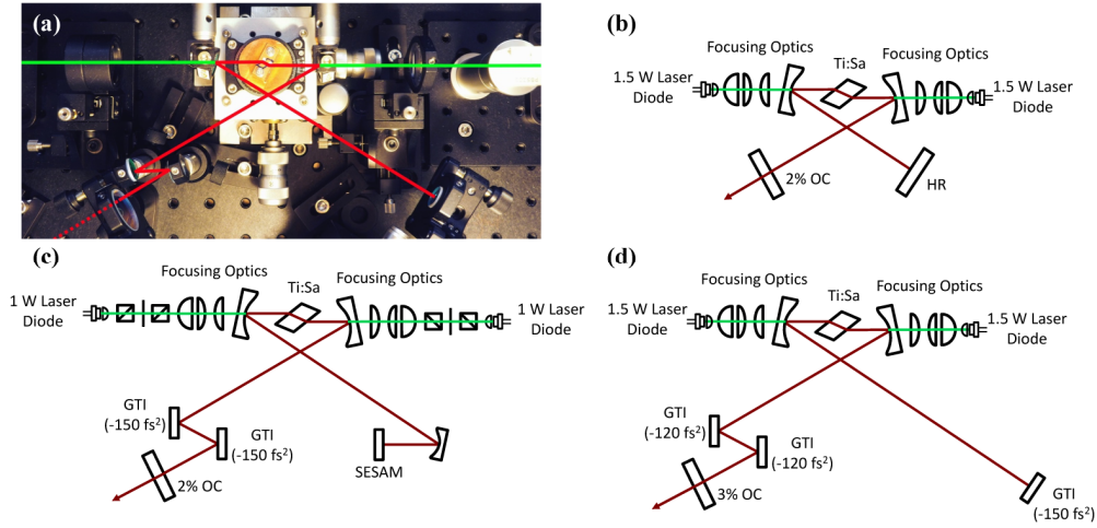
Fig. 1. (a) Cavity picture with pump beam drawn in green and the oscillating laser beam in red. Laser setup for (b) CW, (c) SESAM mode-locked operation, (d) KLM operation.
