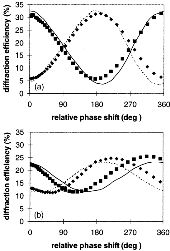
Fig. 4. Measured and calculated diffraction efficiency (in percent) as a function of the relative phase \beta in degrees for the +1 and -1 orders for (a) TM and (b) TE illumination. The measured diffraction efficiencies are shown as filled squares for the +1 order and as filled diamonds for the -1 order; the calculated values are shown as solid and dashed curves for the +1 and -1 orders, respectively.
