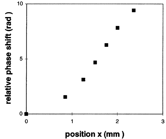
Fig. 3. Relative phase shift between the two basis functions versus position x , as determined from AFM measurements.
