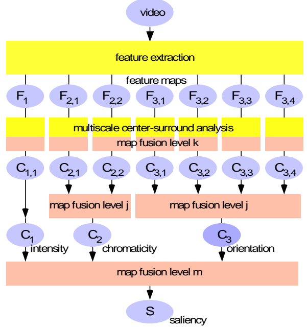
Figure 1: Saliency model of visual attention
