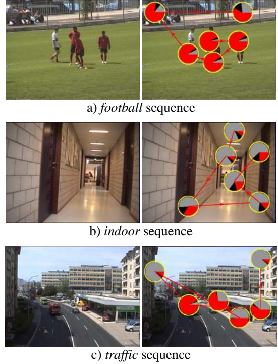
Figure 3: Example frames of three video sequences and the related 6 spots of attention; the cheese diagram indicates the spot percentile contribution to saliency of intensity (black), chromaticity (red) and orientation (grey)
