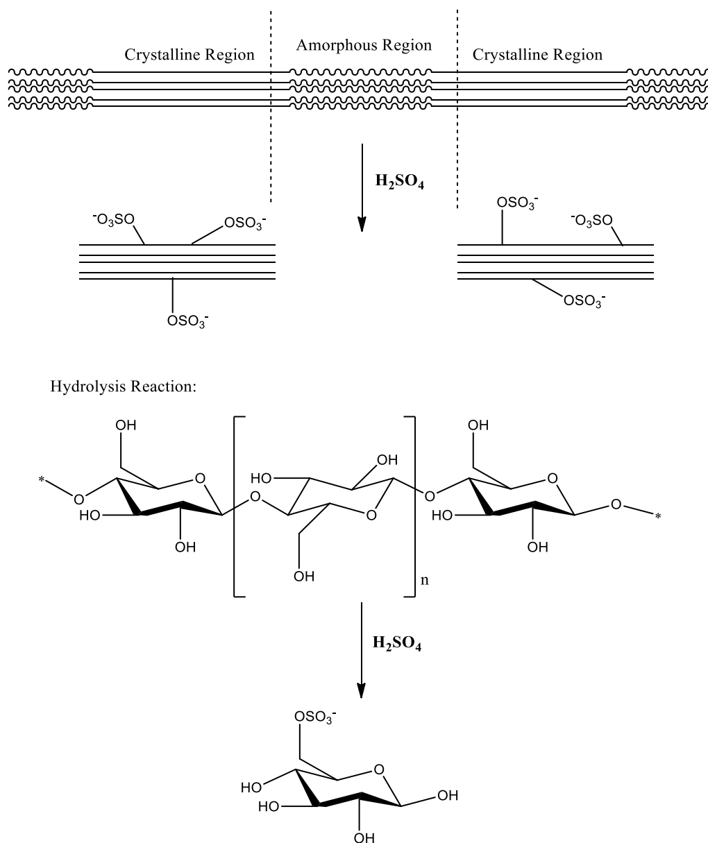
Figure 10 - Schematic representation of the hydrolysis of amorphous and crystalline cellulose with H_2SO_4 , and consequent sulfonation.
