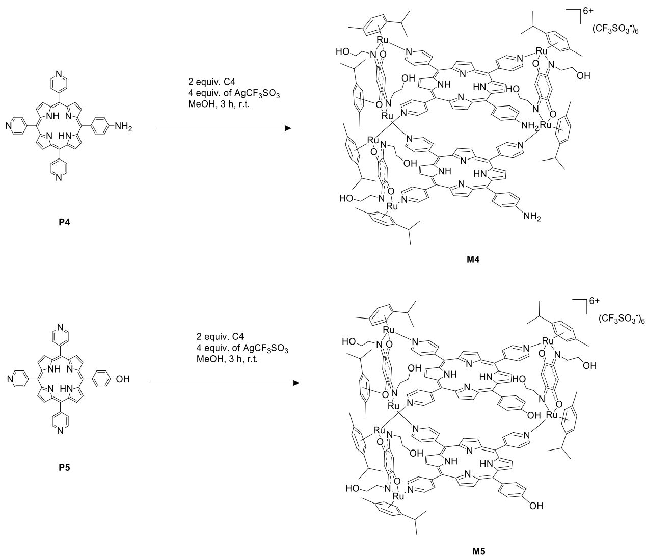
Scheme 2 - Overview of the synthetic route for the metalla-macrocycle assemblies M4 and M5
