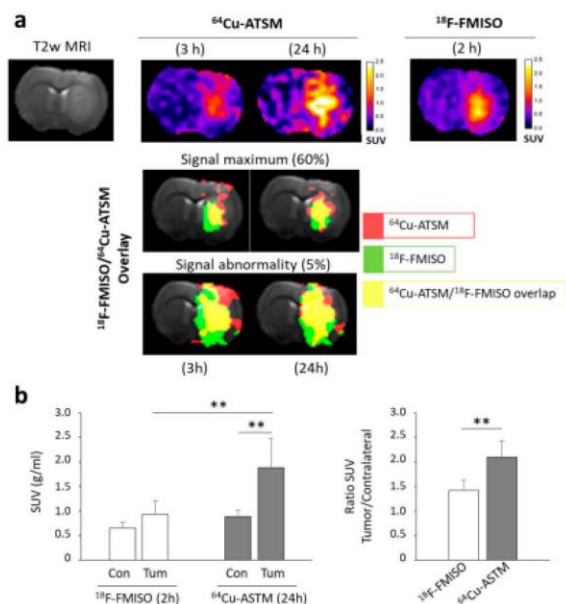
Figure 16. Studies showing the relationships between the retention of [ ^{18}\text{F} ]FMISO and [ ^{64}\text{Cu} ]Cu(ATSM) and hypoxia. (a) Coregistration of the [ ^{18}\text{F} ]FMISO PET signal (2 h postinjection) with the [ ^{64}\text{Cu} ]Cu(ATSM) PET signal (3 or 24 h postinjection). (b) [ ^{18}\text{F} ]FMISO and [ ^{64}\text{Cu} ]Cu(ATSM) uptake was evaluated at 2 and 24 h after radiotracer injection, respectively. 260
