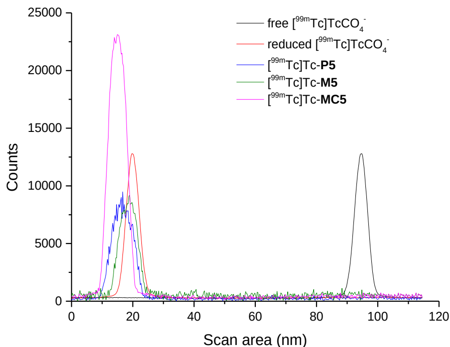
Figure 20 - Radiochemical data of free, reduced [ 99m Tc]TcO 4 - , and radiolabeled compounds. The radio-iTLCs were developed on Whatman 1 MM with acetone as the mobile phase, RCC 99.0%.
