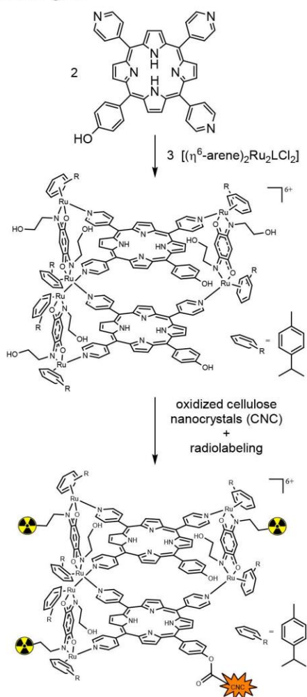
Scheme 4. Synthesis of Cellulose-Metallo-Porphyrin Theranostic Agents
