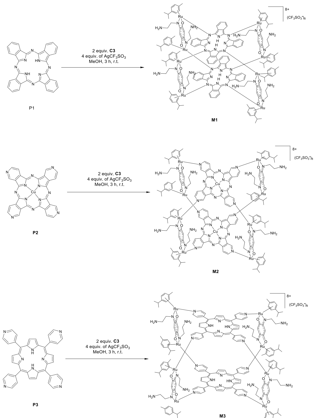
Scheme 1 - Overview of the synthetic route for the metallamacrocyclic assemblies M1-M3 .
