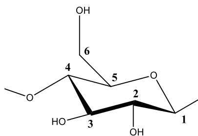
Figure 8 - Numbering system for carbon atoms in anhydroglucose unit of cellulose
