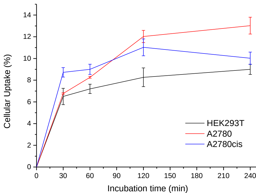
Figure 32 – Cell uptake for [^{111}\text{In}]\text{In-MC5} in the HEK293T, A2780, and A2780cis cell lines up until 4 h. Error bar stands for standard error ( \pm SE), calculated from 3 repeated measurements.
