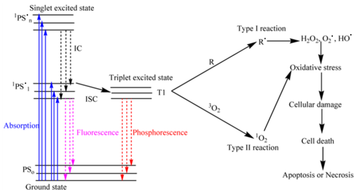
Figure 1 - Modified Jablonski diagram depicting the process of photodynamic therapy. When PSs in cells are exposed to specific wavelengths of light, they are activated, passing from a singlet ground state ( S_0 ) to an excited singlet state ( S_1 – S_n ), which is followed by intersystem crossing to an excited triplet state ( T_1 ). Abbreviations: IC: internal conversion; ISC: intersystem crossing; PS: photosensitizer; ^1PS : Singlet excited photosensitizer; T_1 : Triplet excited state; R: biological substrate; R' : oxidized biological substrate; ^1O_2 : Singlet oxygen; H_2O_2 : hydrogen peroxide; O_2^- : superoxide; HO^\bullet : hydroxyl radical.
