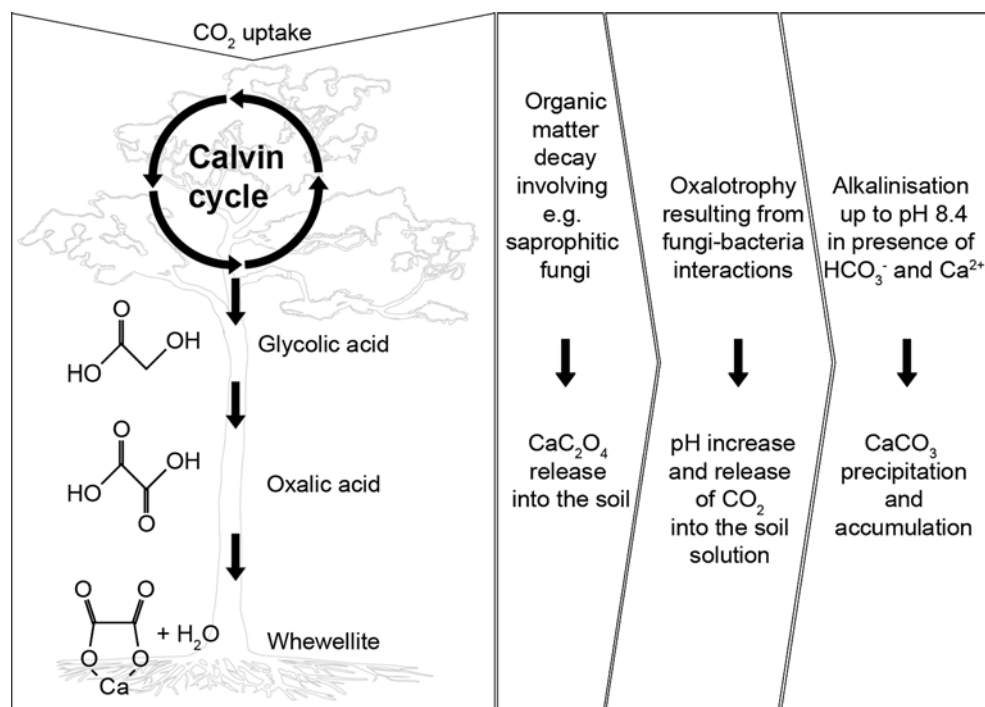
Fig. 1 Schematic representation of the flux of carbon in the oxalate-carbonate pathway. \text{CO}_2 is initially fixed through photosynthesis by an oxalogenic tree that will produce oxalic acid and calcium oxalate (whewellite). Then, calcium oxalate ( \text{CaC}_2\text{O}_4 ) is released into the soil after the decay of organic matter. The consumption of calcium oxalate (oxalotrophy) leads to an increase in soil pH and the final precipitation and accumulation of calcium carbonate ( \text{CaCO}_3 )
