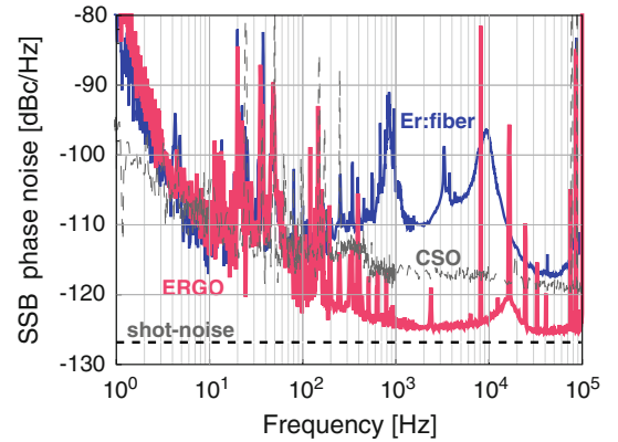
Fig. 5 (Color online) Single-sideband (SSB) phase noise PSD of the 10-GHz microwave generated with the ERGO comb and with a commercial Er: fiber comb for comparison, both evaluated against ULISS. The dashed gray curve shows the phase noise of a CSO obtained in an early comparison between two similar oscillators. Since this time, the short-term stability of ULISS has been improved so that its phase noise in our experimental conditions is very likely lower. The horizontal dashed line indicates the estimated shot-noise floor in the photo-detection of the ERGO comb pulse train. With an incident optical power of \sim 10 mW, the generated photocurrent was \sim 5 mA and the amplitude of the microwave signal at 9.9 GHz was about -34 dBm
