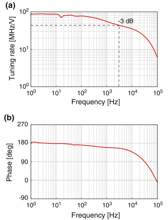
Fig. 2 (Color online) Transfer functions in amplitude (a) and phase (b) of the PW-ECL frequency for injection current modulation applied via the driver input voltage. The -3 dB bandwidth (in amplitude) is \sim 3 kHz
