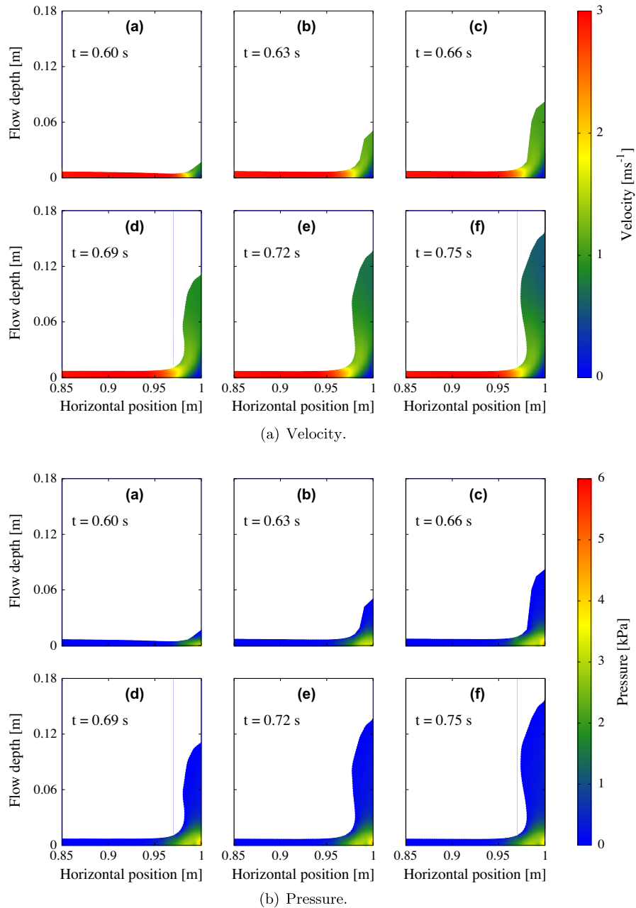
Fig. 10. Snapshots of the evolution of the velocity, |\mathbf{u}| = \sqrt{u^2 + w^2} , pressure p , and flow depth in the vicinity of a perpendicular wall erected at x = 1 m and simulated with the coupled 2D/1D/2D model for a Bingham material with a pressure-independent yield stress \tau_y = 100 Pa.
