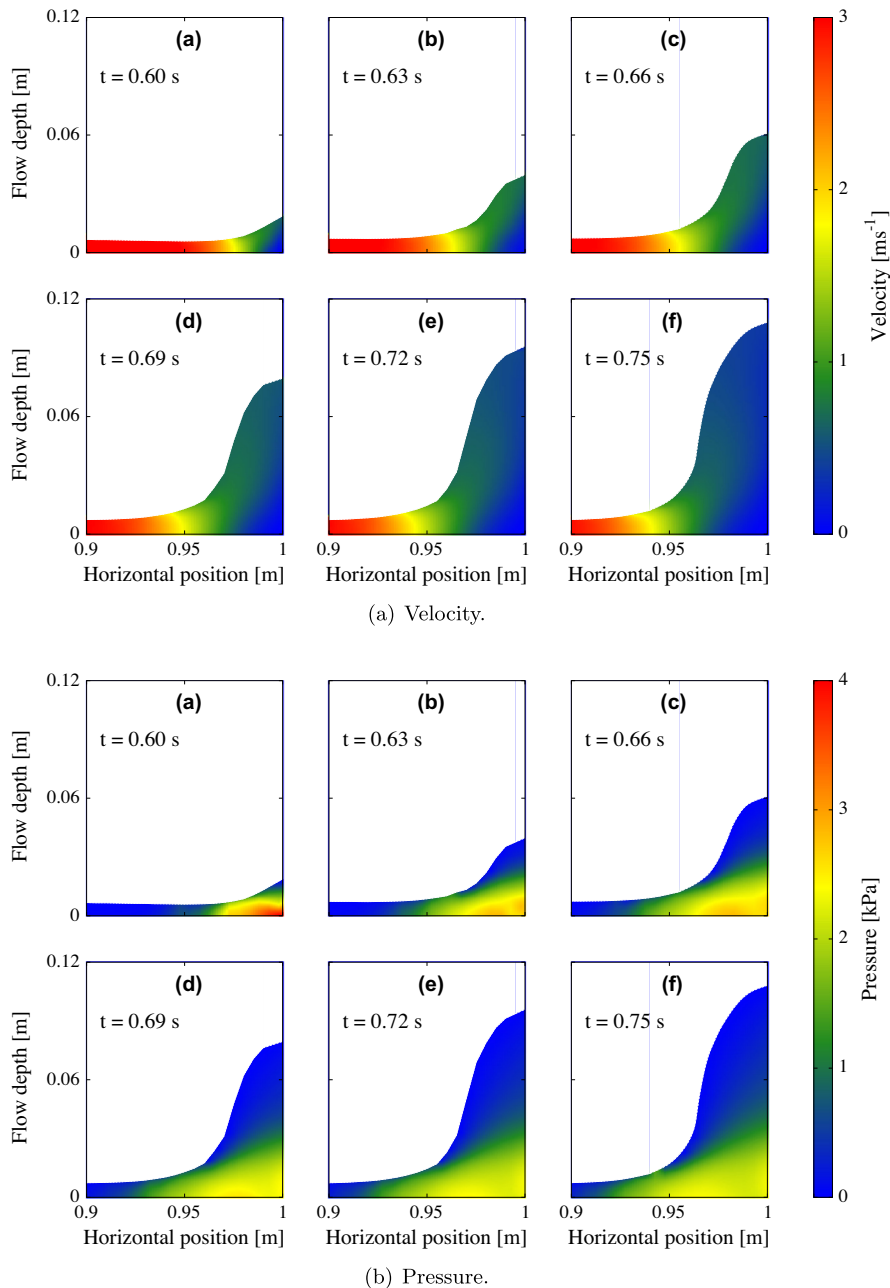
Fig. 9. Snapshots of the evolution of the velocity, |\mathbf{u}| = \sqrt{u^2 + w^2} , pressure p and flow depth in the vicinity of a perpendicular wall erected at x = 1 m and simulated with the coupled 2D/1D/2D model for a granular material with pressure-dependent yield stress \tau_y = \tau_p p with \tau_p = \sin\phi .
