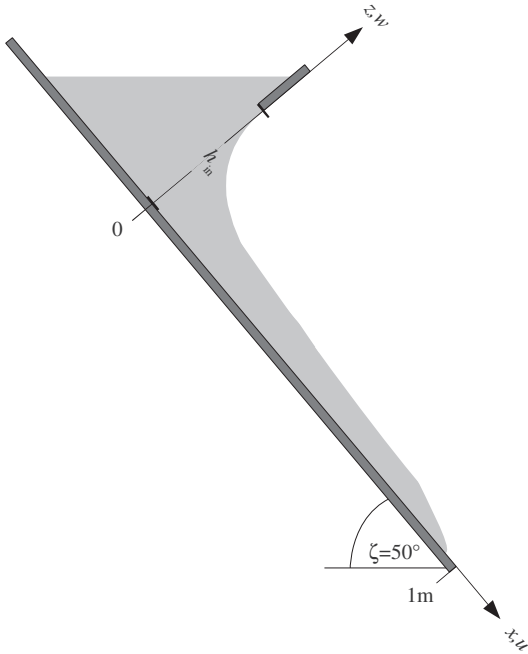
Fig. 1. Side view of an inclined chute with considered coordinate system. The x -axis is aligned in the downslope direction and the z -axis is orientated perpendicular to it. The granular material (depicted in light grey) enters the channel at x = 0 through a silo gate with opening height h_m and flows in the downslope direction. \zeta is the inclination angle of the chute.
