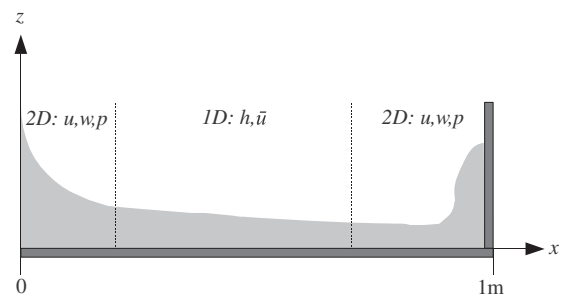
Fig. 2. A possible domain decomposition and the associated field variables for flow along an inclined channel closed by a perpendicular wall at x = 1 m downstream. The 2D model supplies the velocities u , w , and the pressure p . The 1D model provides the flow depth h and the depth-averaged downslope velocity \bar{u} . The dotted lines indicate the 2D–1D, 1D–2D, interface, respectively.
