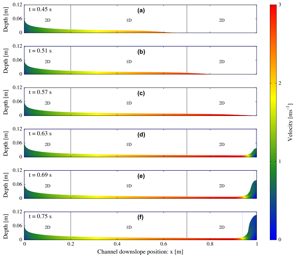
Fig. 8. Snapshots of the evolution of the velocity, |\mathbf{u}| = \sqrt{u^2 + w^2} , and flow depth along the entire channel and simulated with the coupled 2D/1D/2D model. The flow enters the channel at x = 0 . The 2D–1D interface is located at x = 0.2 m and the 1D–2D interface is located at x = 0.7 m (indicated by the grey vertical lines). At x = 1 m a perpendicular wall is erected.
