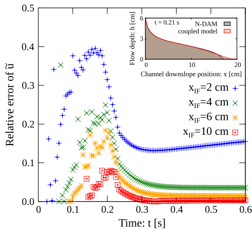
Fig. 14. Relative error of the globally averaged velocity \bar{u} evolving with time for different interface positions x_{IF} . In the inset, the flow depth is shown for the coupled and the full two-dimensional model. The 2D–1D interface position of the coupled model in the inset is located at x_{IF} = 0.1 m.
