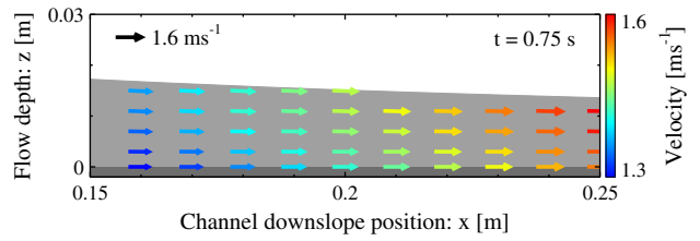
Fig. 5. Velocity field simulated with the full two-dimensional model around x = 0.2 m, which corresponds to the 2D–1D interface in the coupled simulation.
