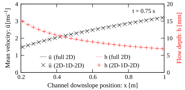
Fig. 6. Mean downslope velocity and height at t = 0.75 s for an undisturbed flow simulated with the full 2D model (lines) and the coupled 2D/1D/2D model (symbols). The 2D–1D interface is located at x = 0.2 m and the 1D–2D interface at x = 0.7 m, respectively.
