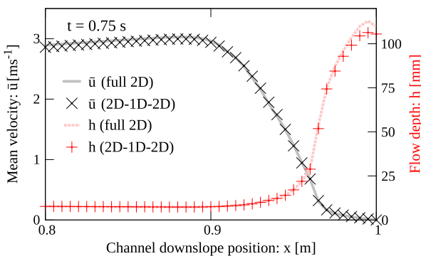
Fig. 11. Mean velocity and height at t = 0.75 s for a flow against a perpendicular wall erected at x = 1 m, simulated with the full 2D model (lines) and the coupled 2D/1D/2D model (symbols).
