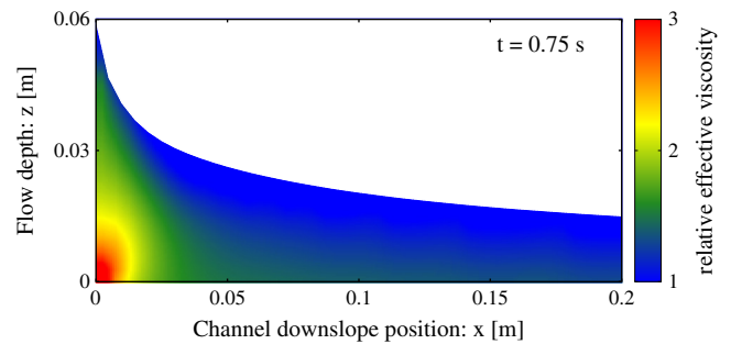
Fig. 7. Ratio of effective viscosity to constant viscosity, v_{eff}/v , near the inlet.
