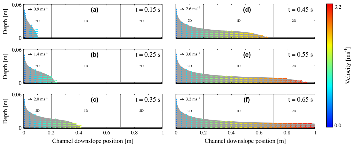
Fig. 4. Snapshots of velocities (arrows) and depth evolutions (background grey) in rapidly flowing granular material down a steep rectangular open channel simulated with the coupled 2D/1D/2D model.
