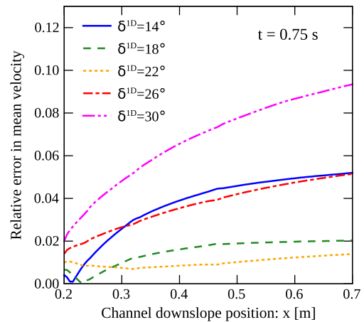
Fig. 12. Relative error of the mean velocity simulated with the coupled 2D/1D model, where the bed friction angle in the 1D subdomain ( \delta^{1D} ) is set independently of the one in the 2D subdomain ( \delta^{2D} = 22^\circ ).
