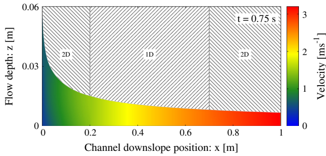
Fig. 3. Simulation of the velocity field, |\mathbf{u}| = \sqrt{u^2 + w^2} , and flow depth of an undisturbed flow with the coupled 2D/1D/2D model. The flow enters the channel at x = 0 . The 2D–1D interface is located at x = 0.2 m and the 1D–2D interface is located at x = 0.7 m (indicated by the grey vertical lines).
