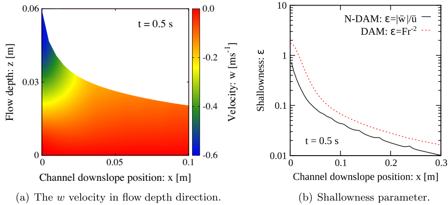
Fig. 13. Simulation of the velocity component in the flow depth direction ( w ) and shallowness parameter, \varepsilon , in the vicinity of the silo inlet (located at x = 0 ). In the full two-dimensional model (N-DAM) \varepsilon is computed by the velocity ratio |\bar{w}|/\bar{u} . In the depth-averaged one-dimensional model (DAM) the shallowness parameter is estimated by \varepsilon = 1/Fr^2 , where Fr is the Froude number.
