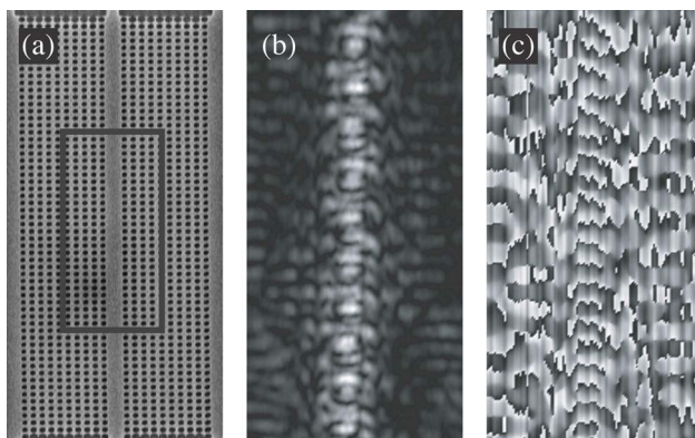
Fig. 3. Straight PC waveguide: (a) top-view scanning electron microscope image of the device (the square outline indicates the approximate SNOM measurement area); (b) SNOM amplitude measurement of the propagating mode in the waveguide over an area of 7\ \mu\text{m} \times 14\ \mu\text{m} ; (c) SNOM phase measurement.
