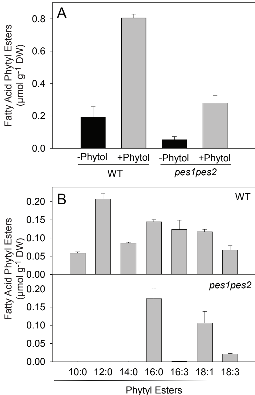
Supplemental Figure 6. Fatty Acid Phytyl Ester Content in pes1pes2 Plants Supplemented with Free Phytol.
