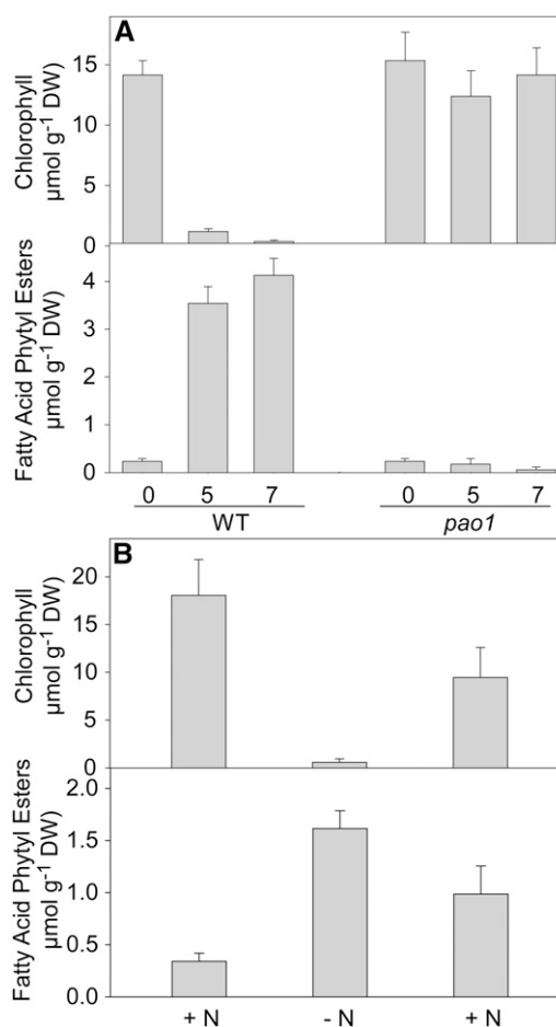
Figure 6. Changes in Chlorophyll and Fatty Acid Phytyl Ester Content during Senescence and Stress.
