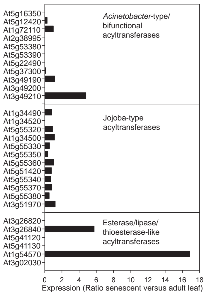
Supplemental Figure 1. Acyltransferase Candidate Genes for Fatty Acid Phytyl Ester Synthesis in Chloroplasts of Arabidopsis . Expression data for acyltransferases of the Acinetobacter/bifunctional, jojoba or esterase/lipase/thioesterase (ELT) families were taken from the Arabidopsis expression database ( www.geneinvestigator.com ). Each bar represents the ratio of expression signals for senescent (experiment ID, AT-00088; three arrays) versus green/adult leaves (798 arrays).
