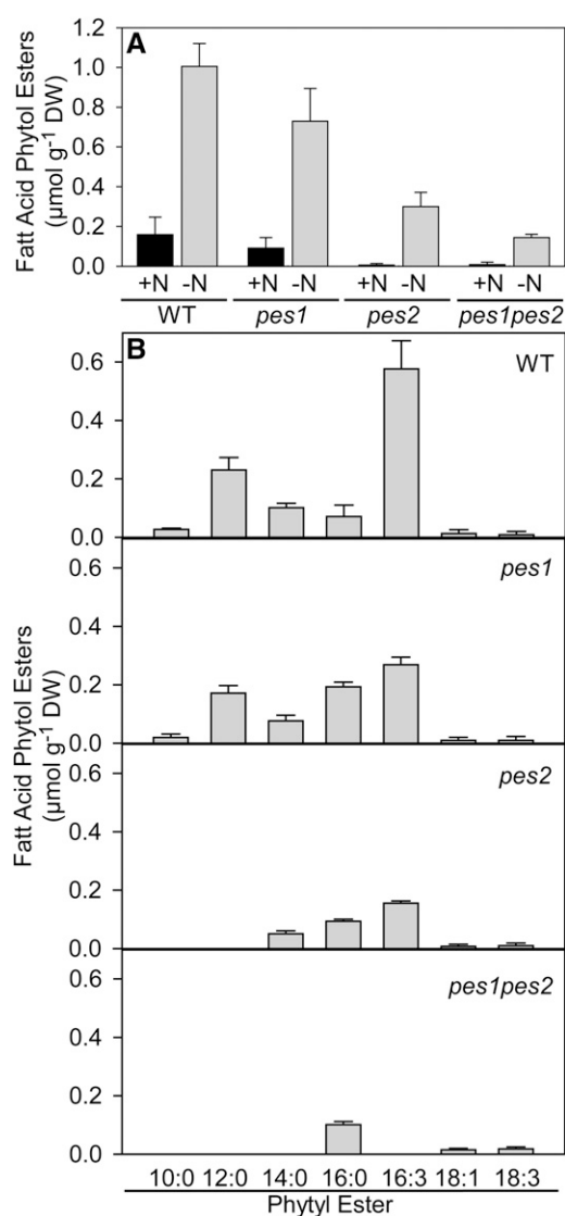
Figure 5. Fatty Acid Phytyl Ester Content of Arabidopsis pes1 and pes2 Mutants during Nitrogen Deprivation.
