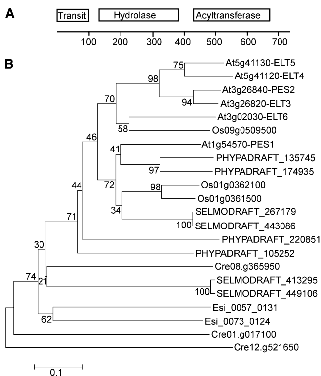
Figure 2. Protein Domains and Phylogram of ELT Sequences.
