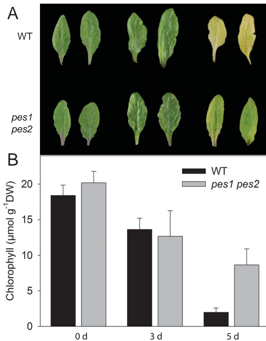
Supplemental Figure 4. Chlorophyll Degradation during Senescence in the pes1pes2 Mutant.
