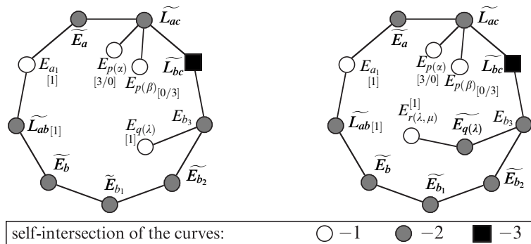
Figure 2. The situation on the surface X . Two curves are connected by an edge if their intersection is positive (and here equal to 1). The positive intersections with \Gamma_1 and \Gamma_2 are in square brackets.
